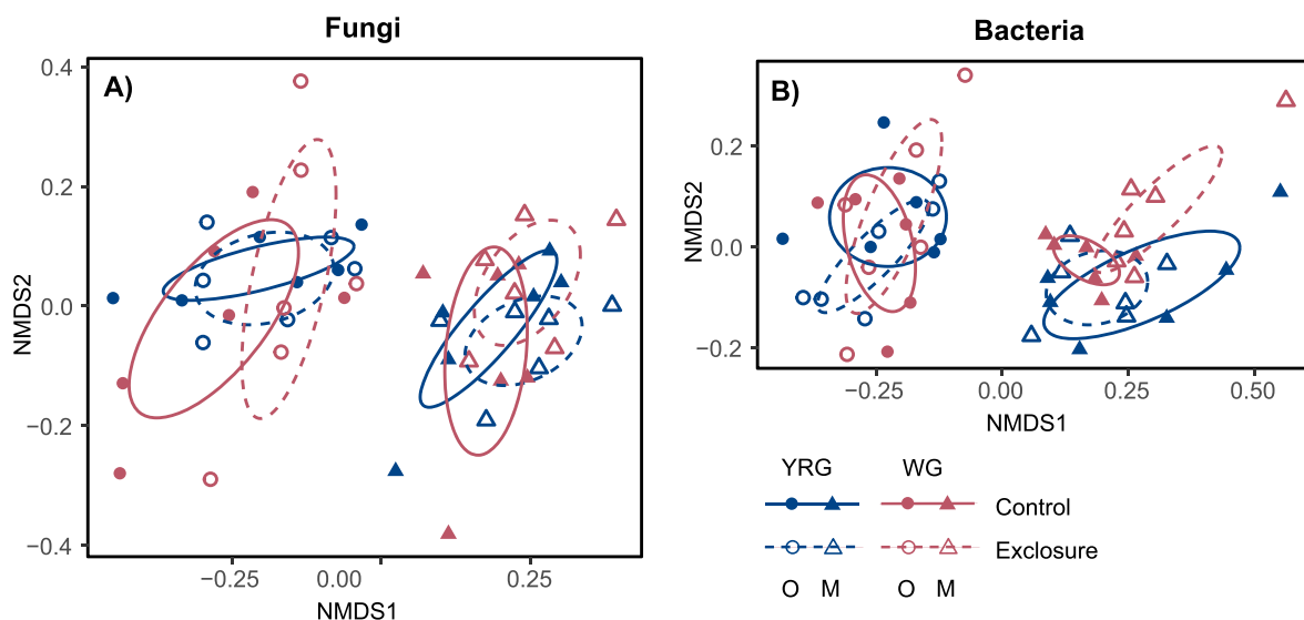
Fig. 2. A non-metric multidimensional scaling (NMDS) of A) fungal and B) bacterial communities in different treatments (control and exclosure), under year-round grazing (YRG) and winter grazing (WG) in organic (O) and mineral (M) soil layers. The ellipses show a 95% confidence interval.
