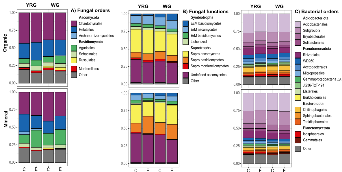
Fig. 1. Mean relative abundances of A) fungal orders, B) fungal ecological functions, and C) bacterial orders in different treatments (control, C and exclosures, E) under year-round grazing (YRG) and winter grazing (WG) regimes in organic and mineral soil layers. Other = undefined and <1\% mean relative abundance orders/fungal functions, EcM = ectomycorrhizal, ErM = ericoid mycorrhizal, Sapro = saprotrophic.
