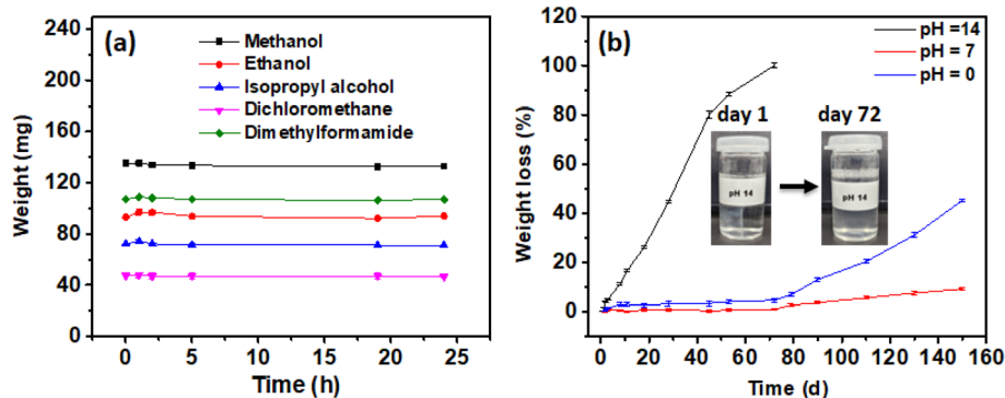
Fig. 4 (a) Chemical stability profile of PCVU exposed in different organic solvents over time, (b) degradation profile of PCVU elastomer over time in different pH aqueous solutions at pH = 0, pH = 7 and pH = 14.
