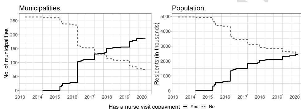
Figure 1: Staggered Adoption of the Nurse Visit Copayment.
