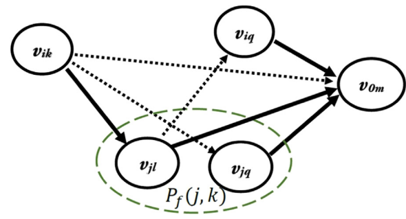
Fig. 3. An illustration of a Br recursion. Consider successive time slots k, l, q and m , s.t. 0 < k < l < q < m , and ships i and j . Thick edges are chosen by Br and dashed edges are other feasible edges. For the choice at node v_{ik} , there were three feasible successor nodes v_{jl}, v_{jq} and v_{0m} . Nodes v_{jl} and v_{jq} belong to a cluster of ship j shown in the dashed circle. While the depot v_{0m} is automatically a candidate node, the cluster is subject to randomization. Based on the probability P_f(j, k) , a single random draw determines whether the nodes in the cluster are accepted as candidates. In this case, the draw was favorable and the node v_{jl} was the best choice at node v_{ik} . - If the dashed edge joining v_{jl} and v_{iq} had been chosen at v_{jl} , then v_{jl} would not be a feasible choice at v_{ik} , because ship i would be in the sub-tour starting at v_{jl} .
