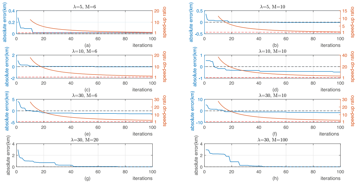
Fig. 6. Comparisons on the average absolute error (over seven days) versus the average speed-up factor over RDP iterations for time horizon |T| = 8 . Figures (a)–(f) relates to six batches of instances with M = 6, 10 shown in Table 1, based on the total execution time and best solutions returned by the ILP solver. Figures (g) and (h) show for two batches of instances with \lambda = 30 and M = 20, 100 the daily average difference of the best solution obtained by RDP by iteration 100 and the current iteration.
