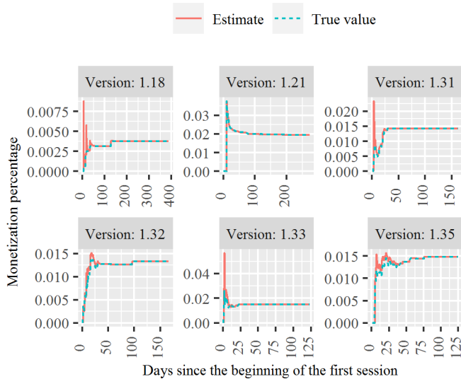
Fig. 6. Estimates of monetization percentage \pi of the real data compared to the true value at each censoring time.
