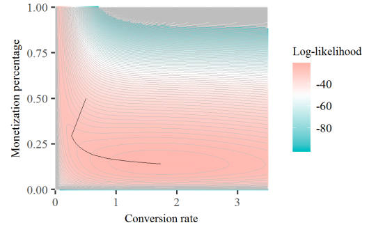
Fig. 2. Values of the log-likelihood as a function of \pi and \lambda . The path of the EM-algorithm iterations is presented as a curve from the initial guess \Psi^{(0)} = (0.5, 0.5) to the maximum likelihood estimate (\hat{\pi}, \hat{\lambda}) = (0.1, 1.7) .
