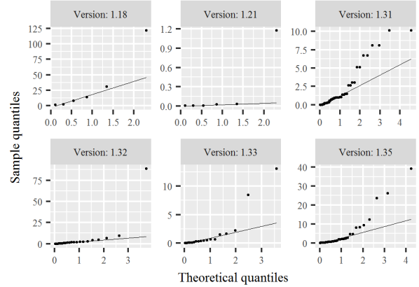
Fig. 5. Q-Q-plots of the event times of each version.
