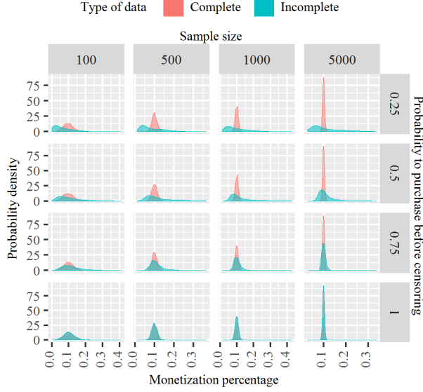
Fig. 3. Simulated estimates of monetization percentage \pi .
