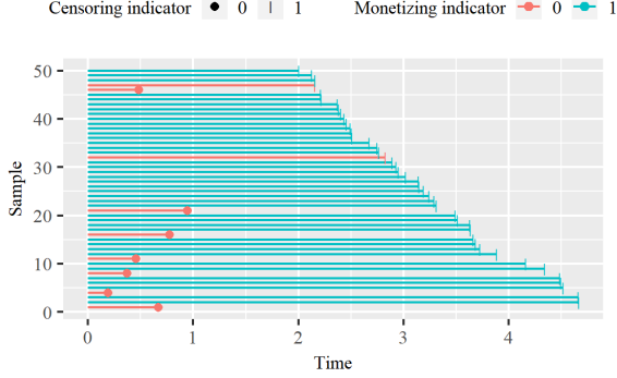
Fig. 1. Simulated data example with 50 players: 9 monetizing and 41 unmonetizing. The data was generated with parameters (\pi, \lambda) = (0.1, 1.0) .
