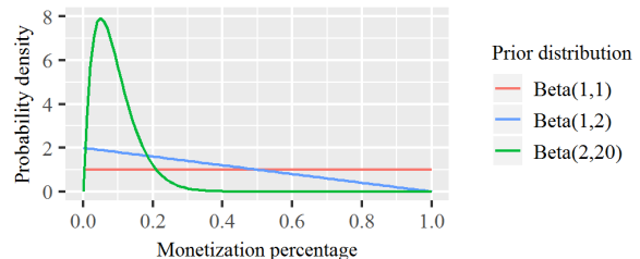
Fig. 7. Possible prior distributions for the monetization percentage \pi .
