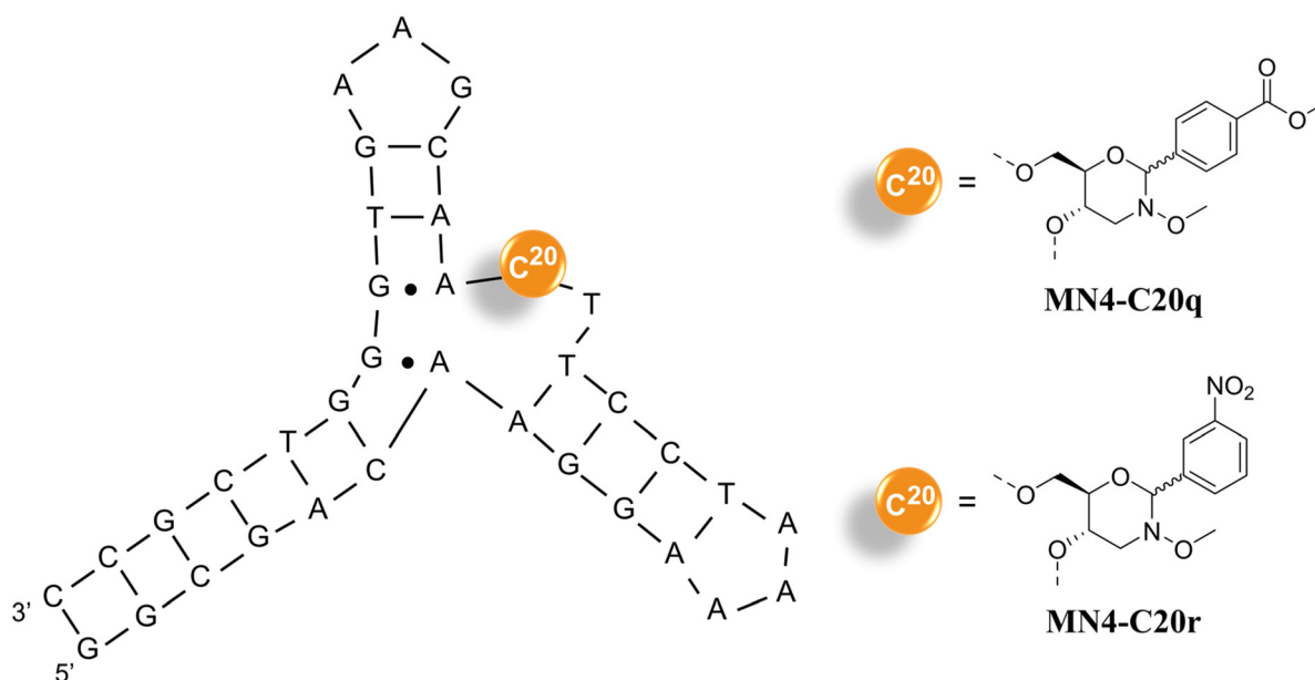
Fig. 2 Structures of MN4-C20q and MN4-C20r .
