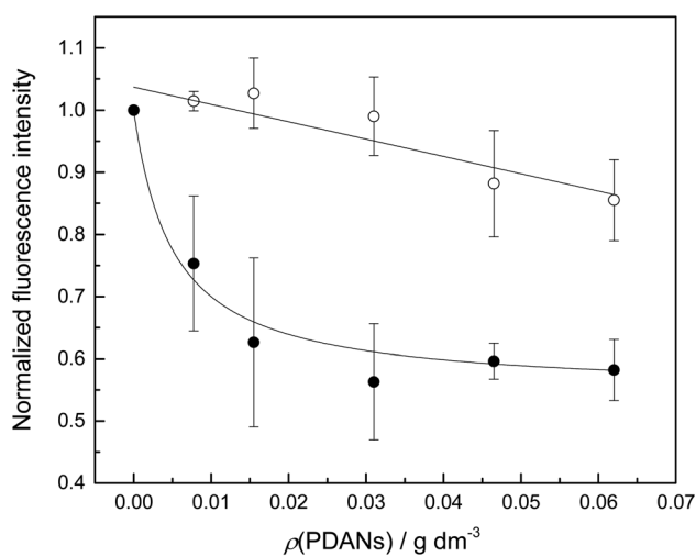
Fig. 1 Fluorescence emission of oligonucleotides ON1c (○) and ON1c-Hg (●) as a function of PDAN concentration; T = 25 °C; \text{pH} = 7.4 (20 mM cacodylate buffer); I(\text{NaClO}_4) = 0.10 M; [oligonucleotides] = 10 nM; \lambda_{\text{ex}} = 493 nm; \lambda_{\text{em}} = 517 nm.
