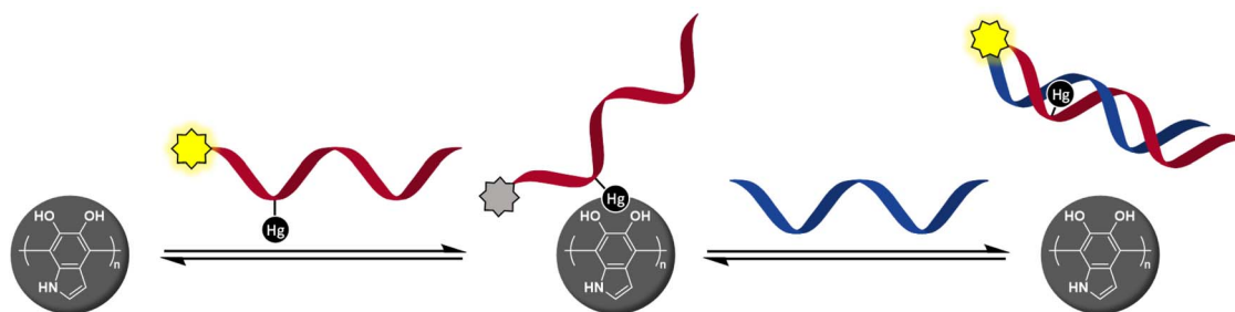
Scheme 1 Hg(II)-promoted adsorption of a fluorescently tagged oligonucleotide probe quenches emission and hybridization with a target sequence restores it.
