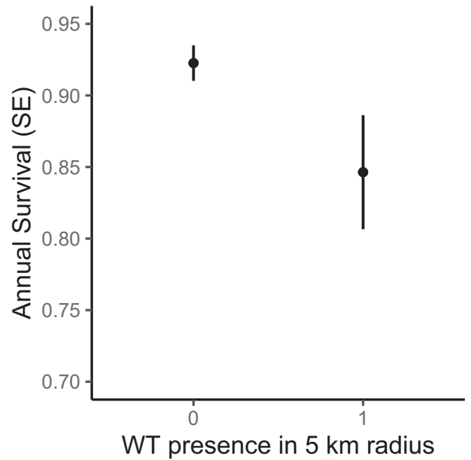
Fig. 2. Annual apparent survival rates ( \Phi ) in relation to presence or absence of wind turbines (WT) in a 5 km radius. The top model for annual apparent survival included in addition to wind turbine proximity also resighting probability ( \rho ) with time (factor, 2010–2022), sex (factor, 'female' or 'male'), observation type (factor, 'visual' or 'genotype'), number of years a nest had been visited over the observation period (numeric, 2–11), mean latitude and mean longitude of all nests an individual had been seen (both numeric) and nest status in a year (factor, 'unknown', 'inactive', 'active' or 'successful nesting attempt'). Error bars depict standard error.
