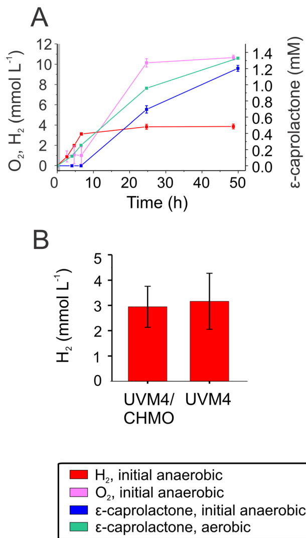
Fig. 5 Stepwise production of H 2 and \epsilon -caprolactone. (A) Production of H 2 (red), O 2 (pink) and \epsilon -caprolactone (blue) under microoxic (initial anaerobic) conditions by the UVM4/CHMO clone 15. To compare the effect of anaerobiosis on biotransformation, the production of \epsilon -caprolactone under an air atmosphere is presented (see the green curve). The grey area in the beginning signifies the time when the vials were under ambient light (2–4 \mu\text{mol photons m}^{-2} \text{s}^{-1} before moving them to the experimental light conditions). (B) Accumulation of H 2 by UVM4/CHMO clone 15 and by the background strain UVM4 after 48 h of incubation. The panel A is a representative experiment with technical repeats. The panel B shows 2–3 biological replications including three technical repeats.
