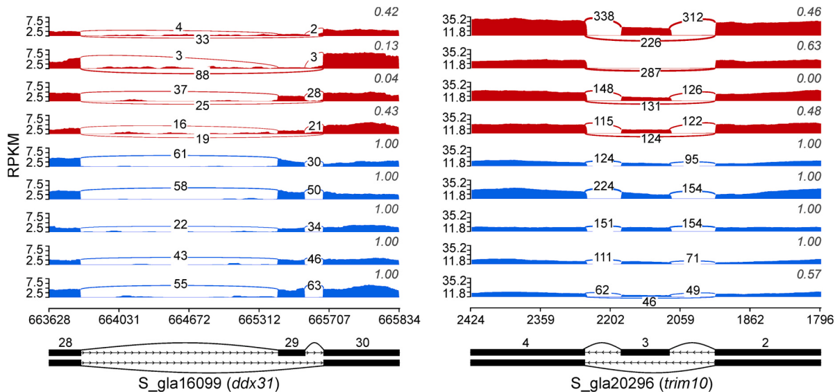
Fig. 5. Sashimi plots showing differential exon and splice junction usage during exon skipping between albino (red) and normally pigmented (blue) S. glanis at the S_gla16099 ( ddx31 ) and S_gla20296 ( trim10 ) genes in skin tissue. Genomic locations are shown on the X-axis, and the transcription intensity, measured as RPKM (reads per kilobase per million mapped reads), is presented on the Y-axis. The arcs connecting exons indicate junction reads. The numbers of junction reads are shown on top of the arcs. The grey numbers in italics on the right indicate inclusion level, i.e., the proportion of normalized read counts in the neighbourhood of the respective exon, which indicates a splicing event, where the exon was included in the final processed mRNA transcripts. (For interpretation of the references to colour in this figure legend, the reader is referred to the web version of this article.)
