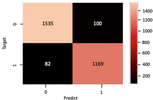
FIGURE 3. Confusion matrix.
