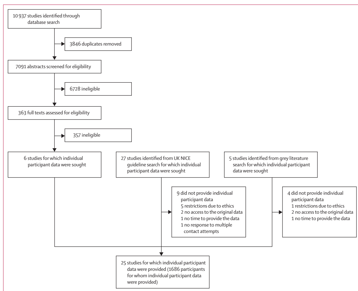
Figure 1: Study selection
