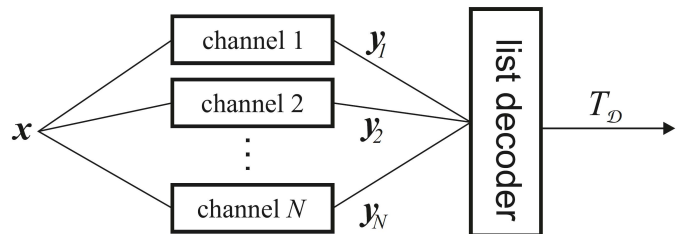
Fig. 1. The Levenshtein's sequence reconstruction.
