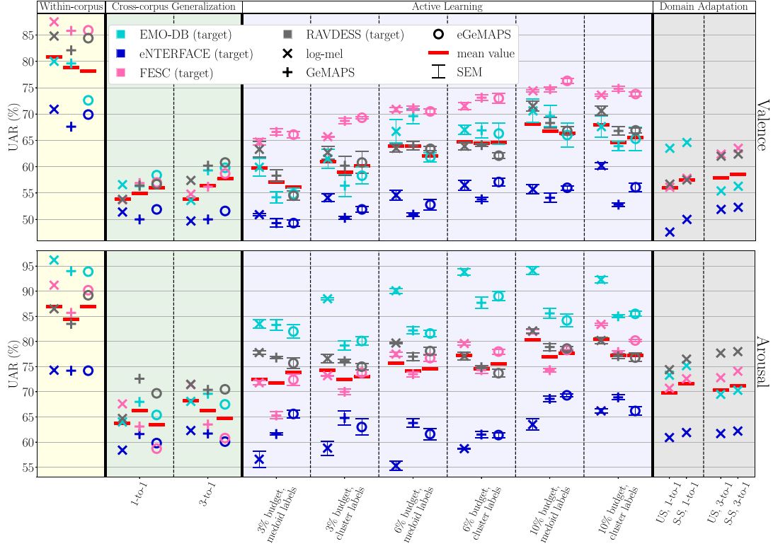
Fig. 4. The unweighted average recall (UAR) performance scores of the simulation experiments for valence (top) and arousal (bottom). The result of each individual experiment is reported for each test corpus and for all three features, with the exception of only using log-mel features in the DA experiments. In the 1-to-1 CCG and DA results, the reported value of each simulation corpus is the mean value of the results of the three separate 1-to-1 settings where the given simulation corpus is used as the test set/target corpus. For AL experiments, the results are shown with three different labeling budgets (3%, 6%, and 10% of the total number of samples in each simulation corpus) and with either medoid labels or cluster labels being used. Since the medoids are initialized at random in MAL, the average of the classification accuracies of five consecutive experiments is reported together with the standard error of the mean (SEM). In the DA experiments, the results for the unsupervised (US) and semi-supervised (S-S) variant of WDA are given. For all experiments, the mean value of the results of the four simulation corpora is given with a red dash. (For interpretation of the references to color in this figure legend, the reader is referred to the web version of this article.)
