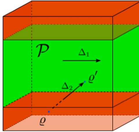
Figure 2. The subset of states sharing a property \mathcal{P} (e.g. coherence) is represented with the green colour. Any measurement distinguishing property \mathcal{P} needs to detect the perturbation operator \Delta_2 , as the direction of \Delta_2 crosses the boundary of \mathcal{P} . This does not happen for the perturbation operator \Delta_1 , which therefore needs not to be detected.
