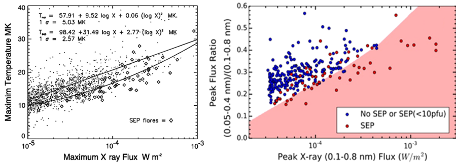
Fig. 14 The maximum temperature (in MK) versus the maximum SXR peak flux (in \text{W/m}^2 ). Flares associated to SEP events are depicted as diamonds, whereas flares not associated to SEP events as dots (from Garcia 2004; left-hand side). The Peak Flux Ratio ( R ) as a function of maximum SXR peak flux (in \text{W/m}^2 ) for flares associated (red dots) and not associated or achieving a peak proton flux < 10 pfu (blue dots) to SEP events (adapted from Kahler and Ling 2018; right-hand side)
