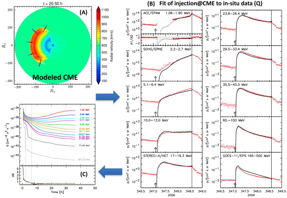
Fig. 11 SOLPENCO outputs for the SEP even on 13 December 2006 SEP event. Panel (A): Evolution of the CME with five observers (dots) including their corresponding magnetic field lines connecting with the shock front displayed in grey. Their corresponding cobpoints are the circles on the shock front. Panel B: Simulated SEP time profiles are then compared to observations. Panel C: Since the calculated time profiles are obtained by using the evolution of the injection rate of shock-accelerated protons at the cobpoint, Q , an iterative procedure is established, aiming at identifying the optimal SEP time profile and from there the transport conditions of SEPs. Assembled from Pomoell et al. (2015)
