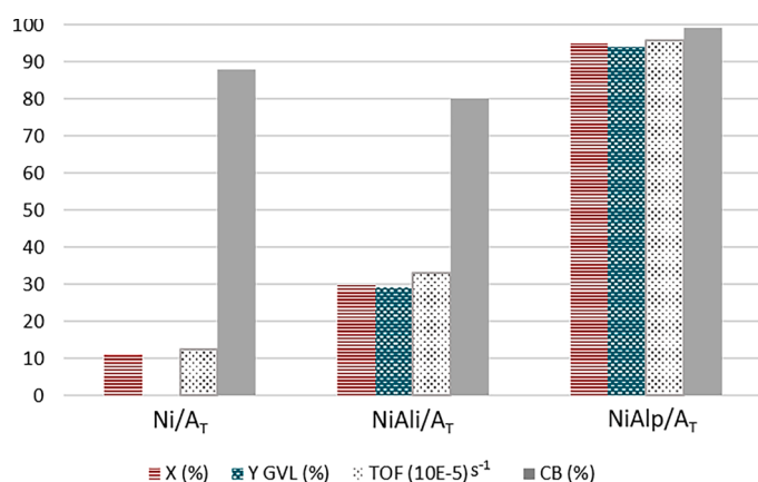
Fig. 9. Transformation of LA to GVL over \text{Ni}/\text{A}_\text{T} , \text{NiAli}/\text{A}_\text{T} , and \text{NiAlp}/\text{A}_\text{T} catalysts. Reaction conditions: 200 °C, 35 bar \text{H}_2 , 4 h, 0.17 M LA, 400 mg catalyst, 50 ml \text{H}_2\text{O} . The relative error of HPLC analysis was generally less than \pm 5 %.
