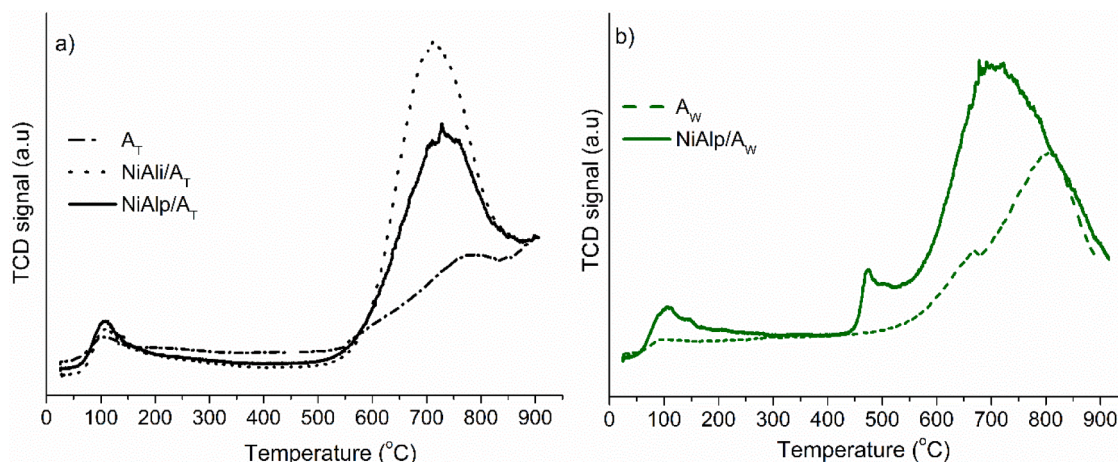
Fig. 8. \text{NH}_3 -TPD profiles of (a) \text{A}_\text{T} , \text{NiAli}/\text{A}_\text{T} , \text{NiAlp}/\text{A}_\text{T} , and (b) \text{A}_\text{W} , \text{NiAlp}/\text{A}_\text{W} samples.
