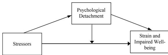
Fig. 1. Stressor-detachment model (Sonnett and Fritz, 2015).
