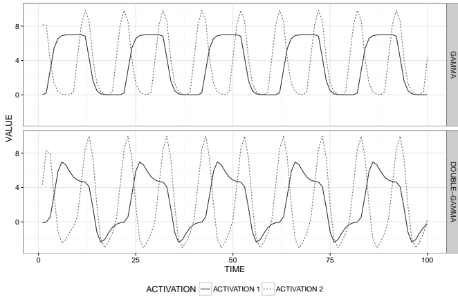
Fig. 1. The activation signals in the simulated data. The upper plot shows the signals of the two activation regions when the option "gamma" is chosen and the lower plot when "double-gamma" is chosen, see Appendix.
