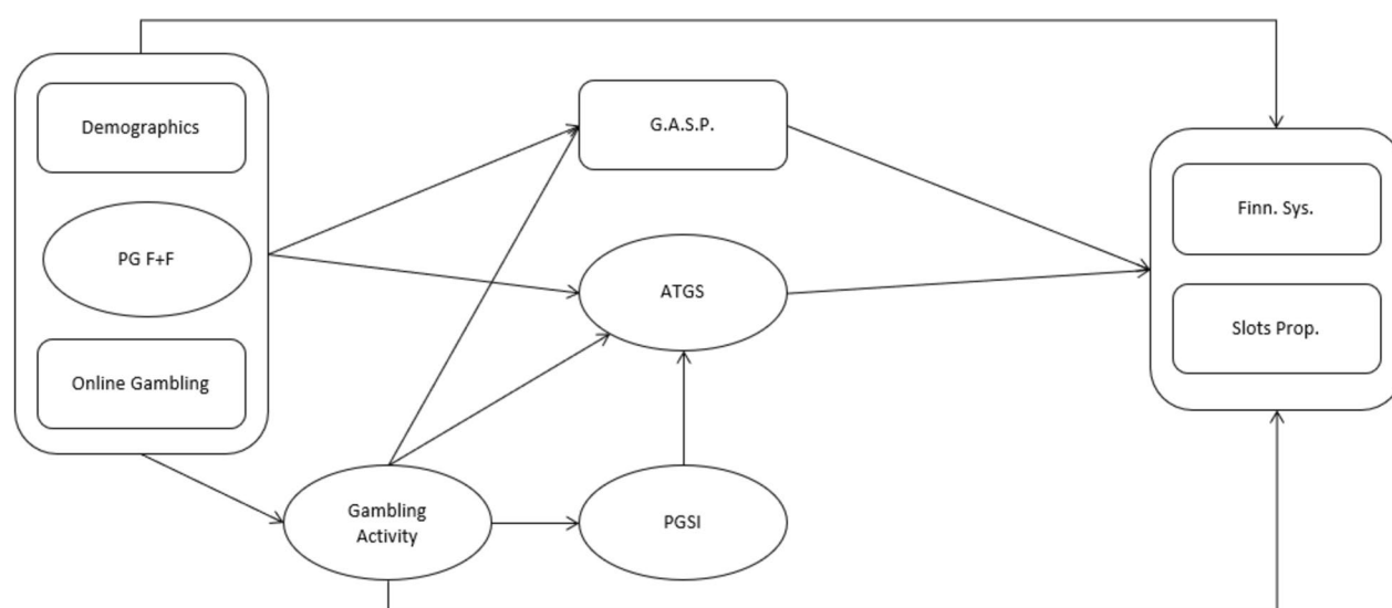
Fig. 1 Research model
