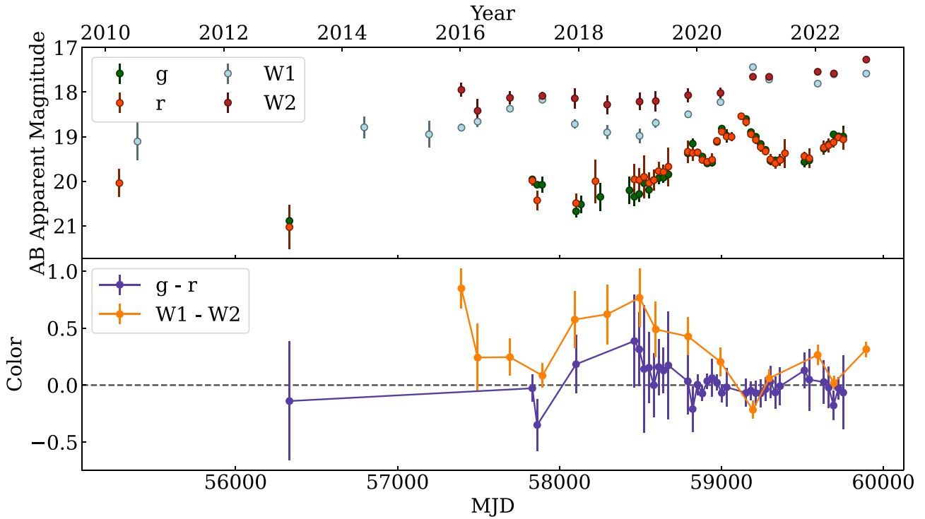
Figure A5. Host-subtracted light curve of AT2017bcc, with the optical and infrared colour evolution plotted below. Each point is the result of binning fluxes to a monthly cadence before converting to magnitudes and calculating colours. All magnitudes are corrected for galactic extinction and host-subtracted using inferred host fluxes from fits to archival SDSS, 2MASS, and WISE photometry, described in Section 4. The optical colours are largely consistent with zero, and are too noisy to show evolution. There may be some evolution in the mid-infrared.
