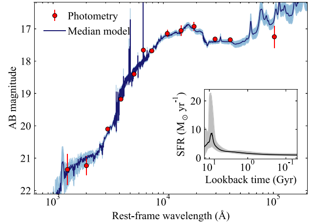
Figure 4. Fit to the archival spectral energy distribution (SED) of the AT2017bcc host galaxy using PROSPECTOR. The inset shows the implied star-formation history. Shaded areas show the 16th and 84th percentiles of the model posteriors.
