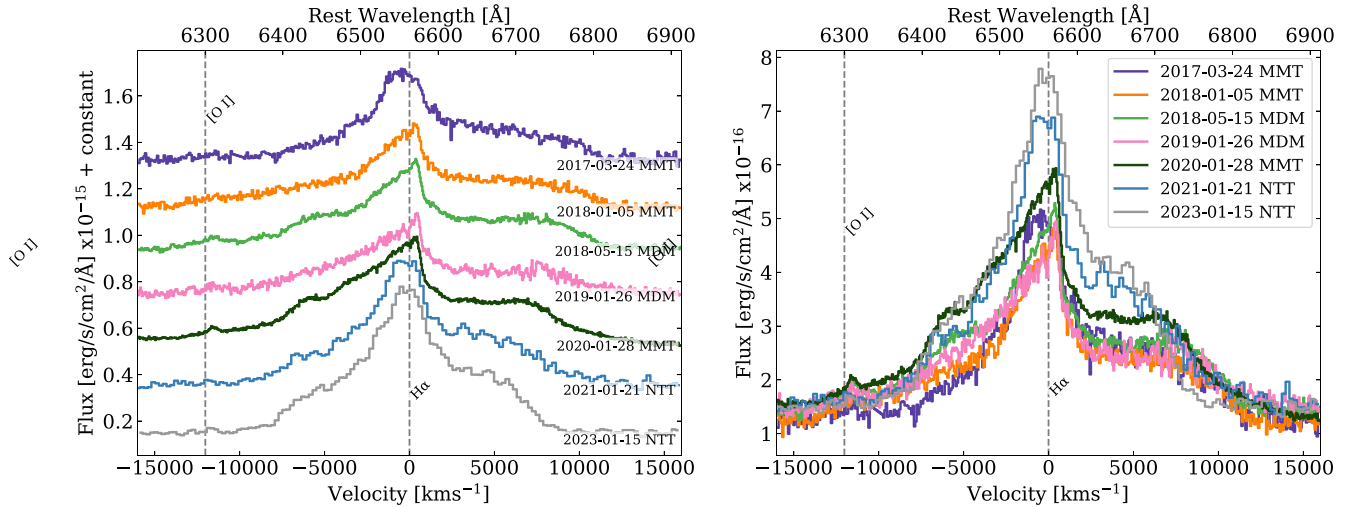
Figure 8. Time-series evolution of the H\alpha emission profile of AT2017bcc. All epochs have been flux-corrected using survey photometry and telluric-corrected. The left and right panels show the same spectra with and without vertical offsets respectively for visual clarity.
