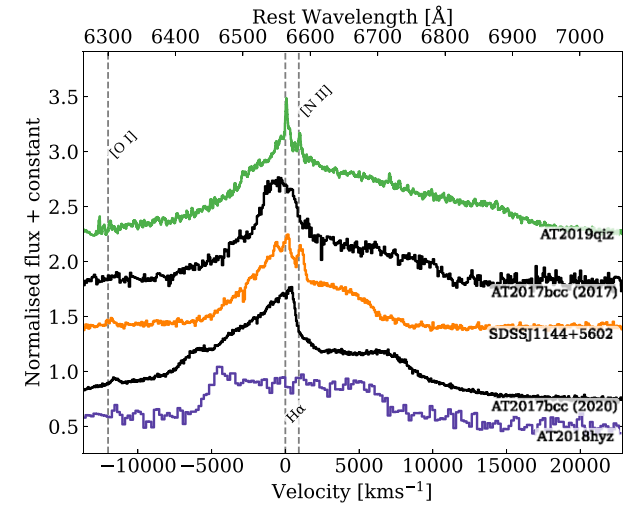
Figure 9. Spectral comparison between two epochs of AT2017bcc (coloured black) and other nuclear transients. The comparison objects were selected from the literature for their similar features to AT2017bcc, and their high signal to noise ratios. All spectra have been normalized for visual clarity. The right panel shows a zoom-in on the H\alpha profiles with alternative normalization, for ease of comparison.
