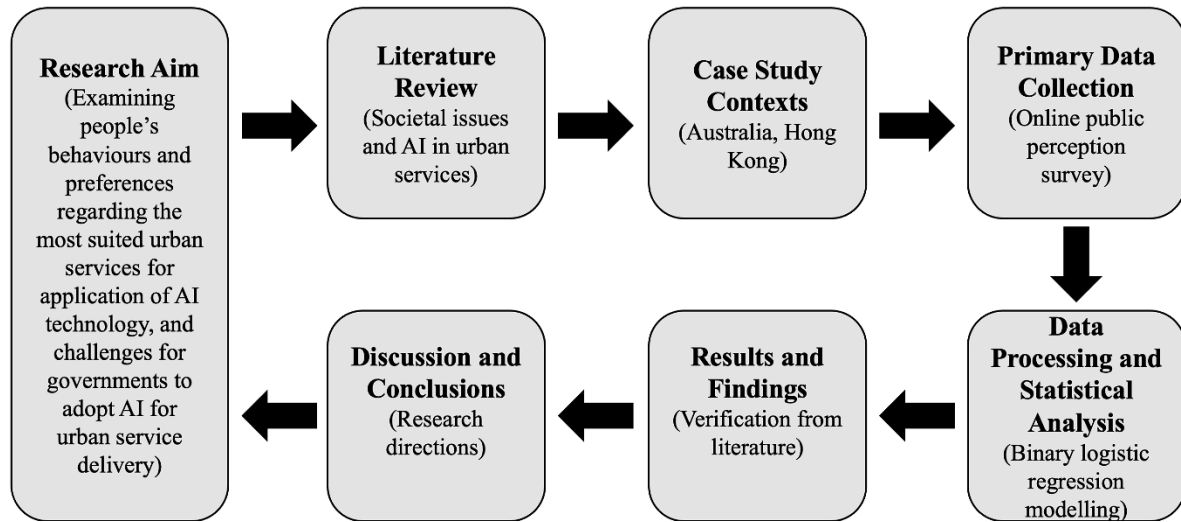
Figure 1. Research flowchart
