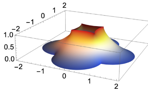
Fig. 5. Potential: m = 1 .
