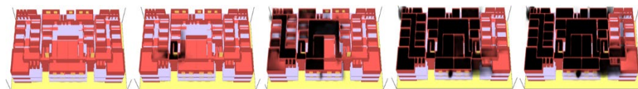
Fig. 4. Smoke flow simulation, as presented in Smokeview visual interface, on the third floor of the building at five different times, each separated by 200 seconds.
