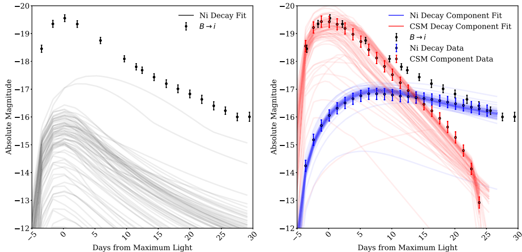
Figure 14. Left-hand panel: Comparison of the light curves produced using MOSFIT for a ^{56}\text{Ni} powered light curve with a limit on the ^{56}\text{Ni} to total ejecta mass fraction of < 0.6 . The optical bolometric light curve points are in black and the fitted light curves with the top 25 percent of scores are shown in grey. Right-hand panel: The ^{56}\text{Ni} model outputs compared to the SE-SN light-curve component identified in Section 3.4. The optical bolometric light curve points are in black and the fitted light curves with the top 25 percent of scores of the ^{56}\text{Ni} fit are shown in blue with the corresponding fitting of the CSM component shown in red.
