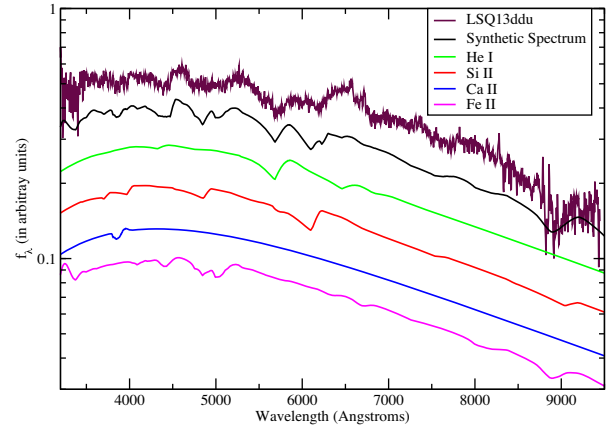
Figure 12. The +9\text{ d} spectrum of LSQ13ddu (purple) along with the best SYNAPPS fit (black). The individual line identifications for the unambiguously determined ionic species of He I (green), Si II (red), Ca II (blue), and Fe II (magenta) are plotted underneath. All have a photospheric velocity of 10\,200\text{ km s}^{-1} . Additional, weaker lines from O I, Co II may also be present, but do not significantly contribute to the spectral fit.
