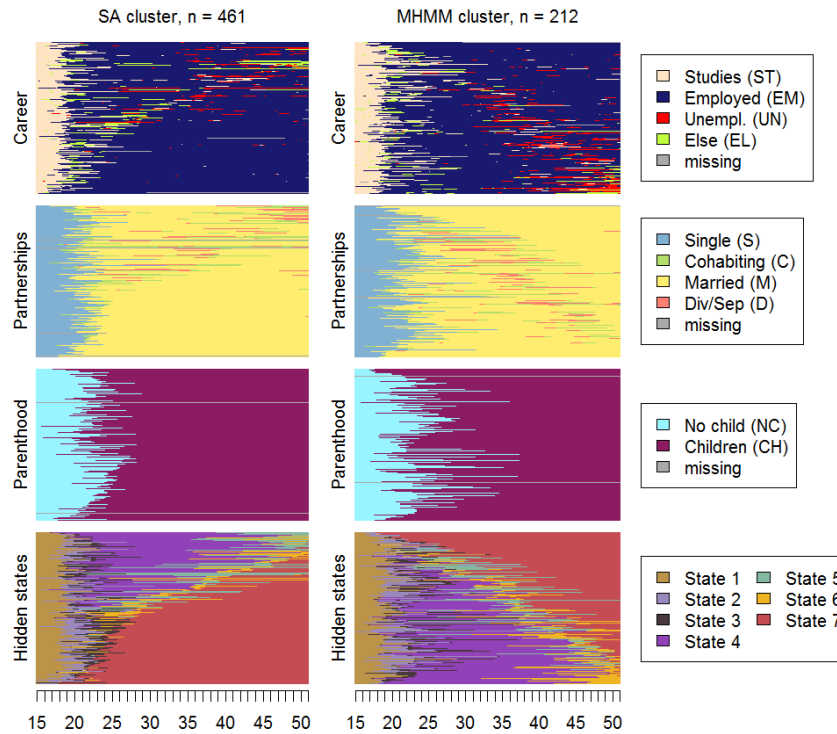
Fig. 7 Comparison of a cluster (Short education and early family) given by SA and the non-estimated MHMM.
