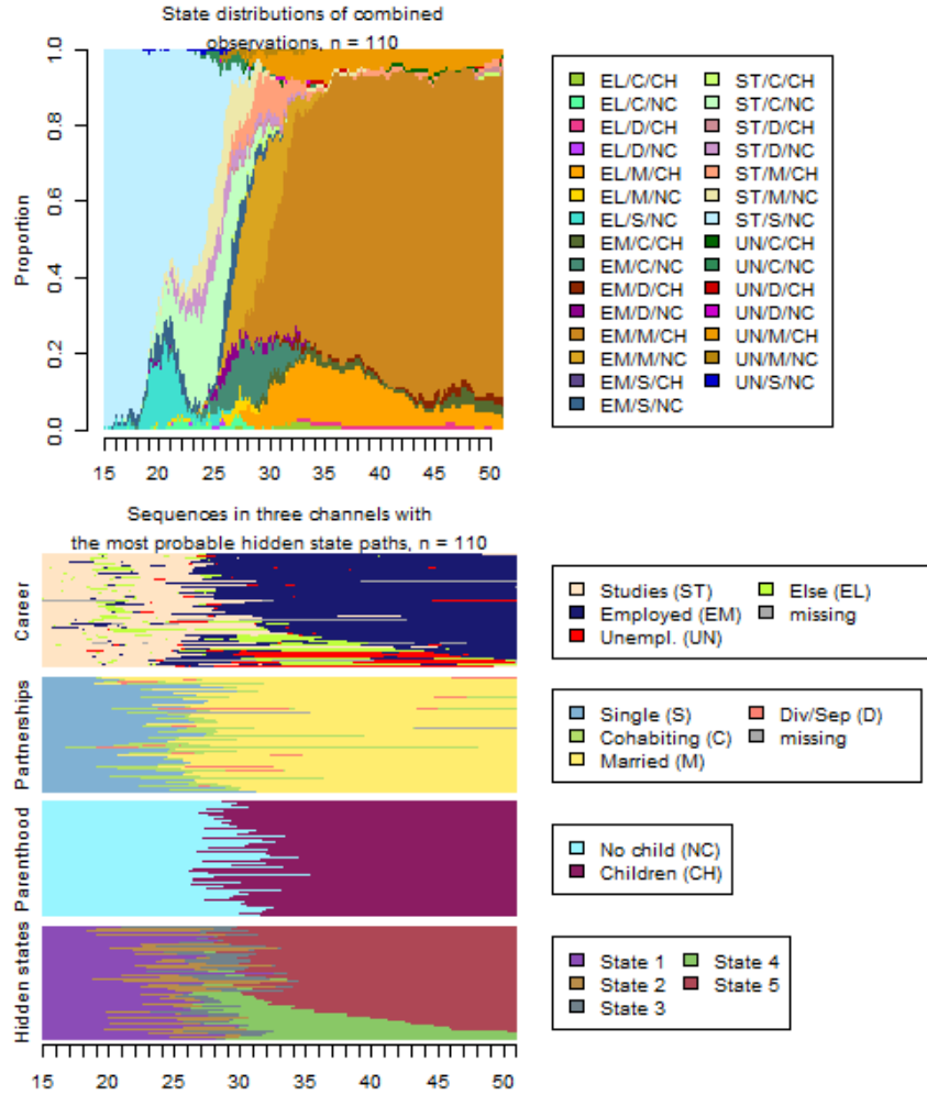
Fig. 3 State distributions of combined observations (top) and sequences of observations in each channel as well as the most probable paths of hidden states (bottom). Sequences are ordered by multidimensional scaling scores. States 1–5 correspond to the hidden states presented in Fig. 1.
