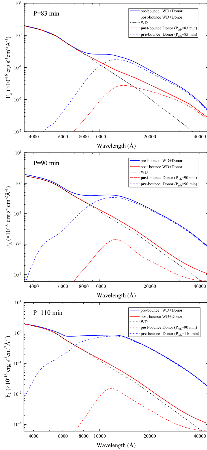
Figure 1: Theoretical SEDs of pre- and post-period-minimum CVs with the orbital periods of P_{orb}=83 min (upper panel), 90 min (middle) and 110 min (bottom) shown together with the SEDs of the WD and the donor star. The SEDs are scaled to the distance of 275 pc.
