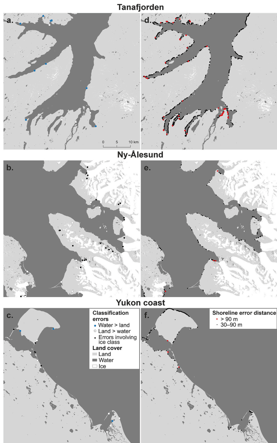
Fig. 15. Distribution of errors in the final coastal land cover data. Panels a.–c. show the distribution of the misclassified reference points and panels d.–f. the shoreline error distances for the time-step 2019–2023 in the three calibration sites.
