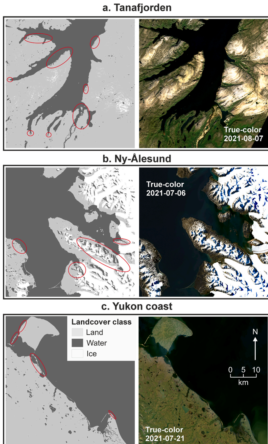
Fig. 13. Land cover and problematic areas after simple threshold-based classification. Panel a. shows land cover classification results based on NDWI and NIR thresholds in 2019–2023 in the Tanafjorden calibration site, panel b. in Ny-Ålesund and panel c. in the Yukon coast. Example areas with notable classification problems are circled on the land cover maps. True-colour Sentinel-2 images are shown for reference.
