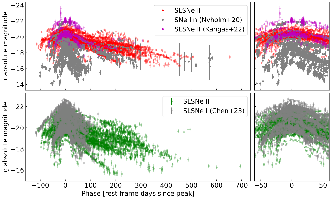
Fig. A.6. Top left panel: comparison of the rest frame r band light curves of our sample of SLSNe II (red dots), the sample of SLSNe II (magenta dots) of Kangas et al. (2022) and the sample of SNe IIn (gray dots) of Nyholm et al. (2020). Bottom left panel: comparison of the rest frame g band light curves of our samples of SLSNe II (green dots) and the SLSNe I (gray dots) sample of Chen et al. (2023). Top and bottom right panels show the same as the respective left panels but constrained to \pm 60 rest frame days from peak.
