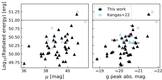
Fig. 11. Total radiated energy of the full sample of SLSNe II. The left panel compares the total radiated energy with the distance modulus and the right panel with the rest g band peak absolute magnitude, shown as black filled markers. Empty sky-blue markers show the corresponding parameters for the ZTF SLSNe II sample presented by Kangas et al. (2022), see Sect. 5.1 for a discussion.
