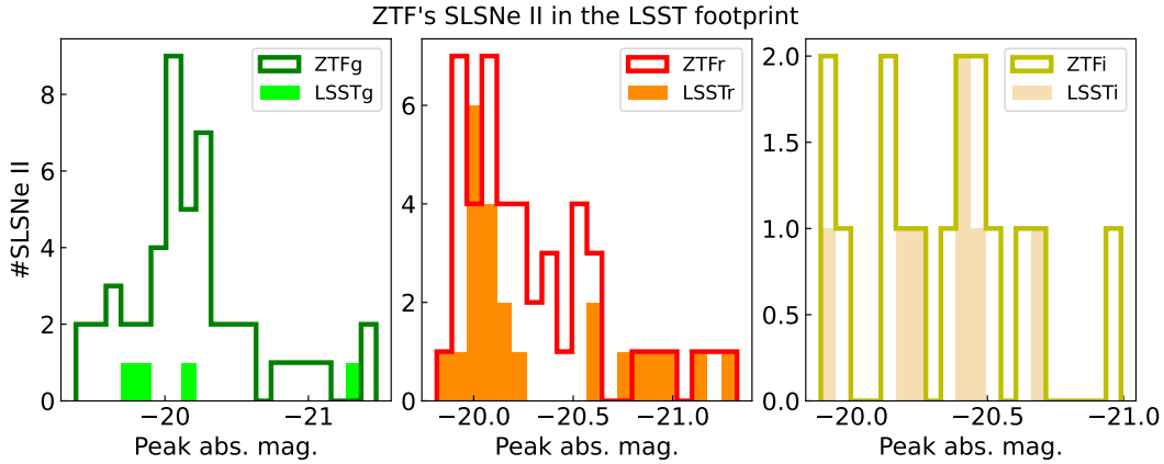
Fig. 16. Distribution of gri (left, center, and right panels, respectively) peak absolute magnitudes as observed by ZTF and LSST.
