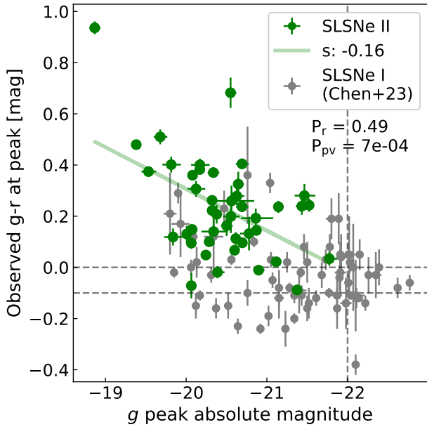
Fig. 8. Observed g - r colors at around g band peak versus rest frame g band peak absolute magnitude of our SLSNe II (green) and the sample of SLSNe I (gray) presented by Chen et al. (2023). In green we include a straight line fit to the scatter plot, the slope ( s ) is indicated in the label of the figure. We also annotate the distribution’s Pearson’s r parameter and associated p value. Horizontal dashed gray lines show the interval between the bluest color of the SLSNe II and color = 0.0 mag. A vertical dashed gray line indicates peak absolute magnitude = -22 mag.
