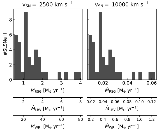
Fig. 15. Mass loss rate ( \dot{M} ) of the SLSNe II for which we can approximate a pseudo-bolometric light curve (see Sect. 3.4) considering a RSG, LBV and WR progenitor. The different mass loss rate ranges are shown in consecutive horizontal axis. The left panel considers v_{\text{SN}} = 2500 \text{ km s}^{-1} and the right panel v_{\text{SN}} = 10\,000 \text{ km s}^{-1} .
