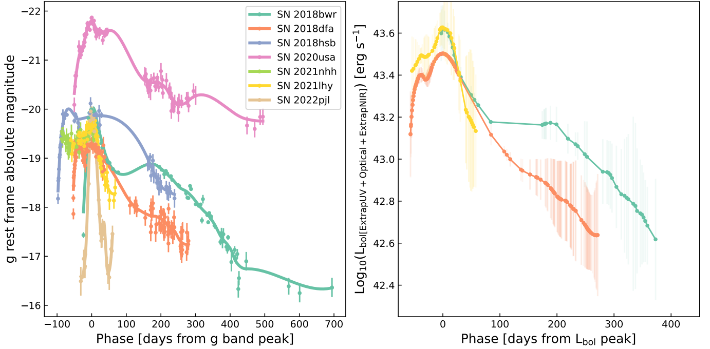
Fig. A.1. SLSNe II with multiple peaks detected visually. Left panel: rest frame g band absolute magnitude with respect to rest frame days since g band peak. Right panel: pseudo-bolometric light curves of multipeaked events with gri band observations.
