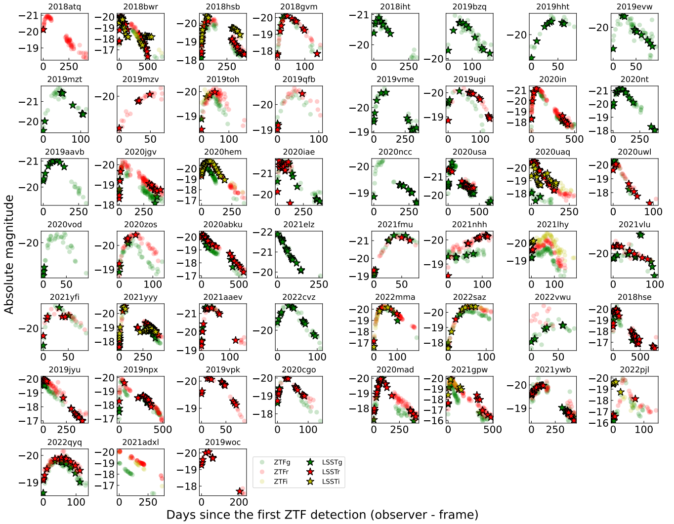
Fig. A.7. SLSNe II gri ZTF light curves (light green, red, and yellow circles, respectively) as observed with the LSST cadence in gri bands (green, red, and yellow stars, respectively).
