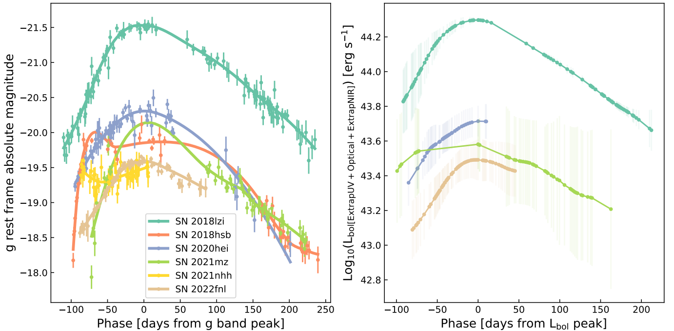
Fig. A.2. SLSNe II with t_{\text{rise},1/e} \geq 80 rest frame days in any of the gri photometric bands. Left panel: rest frame g band absolute magnitude with respect to rest frame days since g band peak. Right panel: pseudo-bolometric light curves of events with gri band observations.
