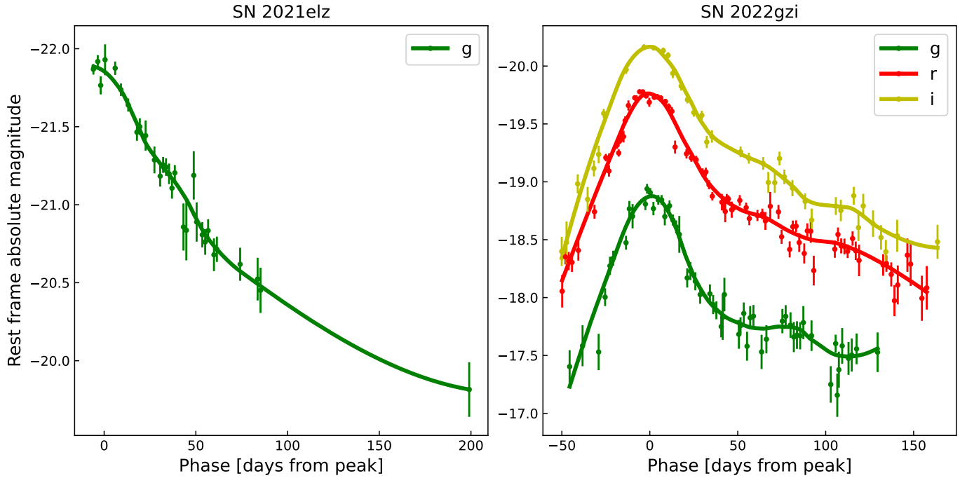
Fig. A.5. Left panel: Light curve of the brightest event in the SLSN II sample. Right panel: Light curves of the faintest event in the SLSN II sample.
