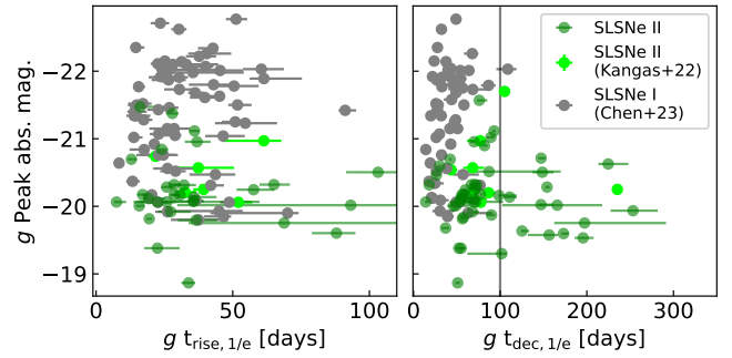
Fig. 13. Comparison of g band timescales versus peak absolute magnitudes for SLSN II and SLSN I. Left panel: g band t_{\text{rise}, 1/e} versus rest frame peak absolute magnitude for our sample of SLSNe II (green circles) and for the SLSN I (gray circles) sample of Chen et al. (2023). Right panel: g band t_{\text{dec}, 1/e} versus rest frame peak absolute magnitude for our sample of SLSNe II (green circles) and the SLSN I (gray circles) sample of Chen et al. (2023).
