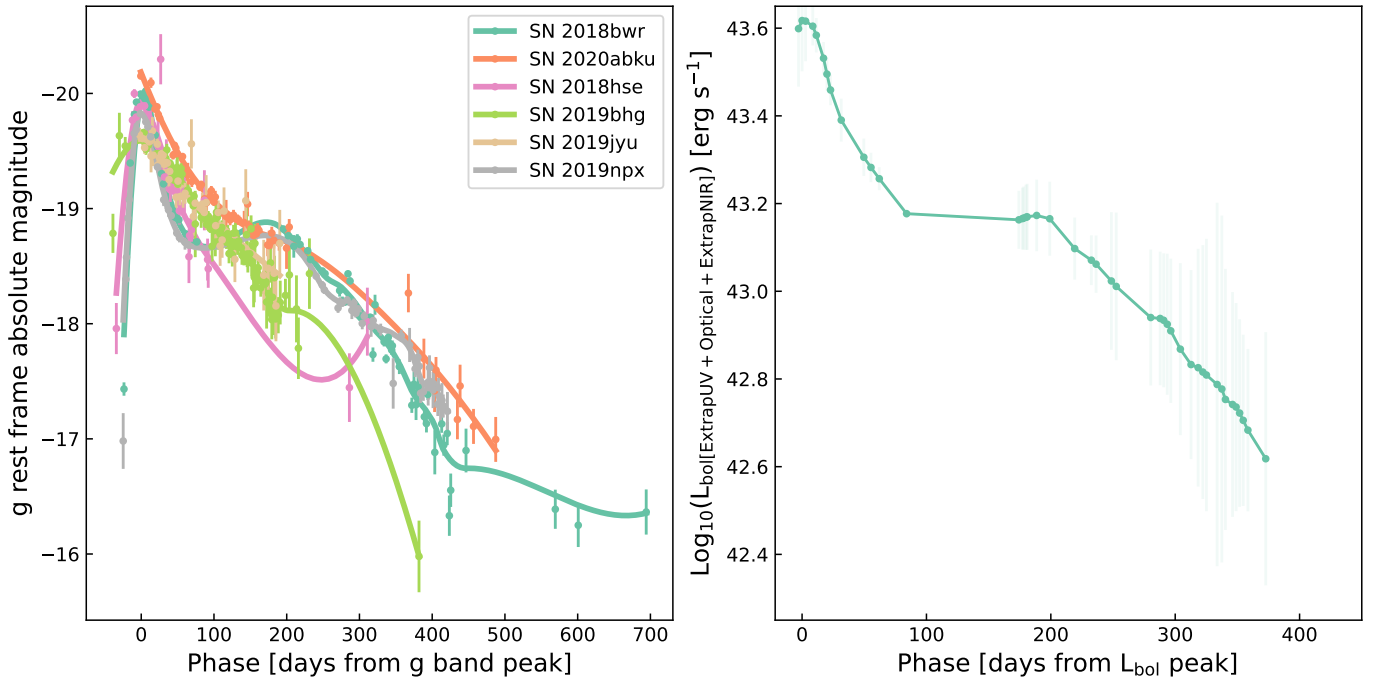
Fig. A.4. SLSNe II with t_{\text{dec},10\%} \geq 365 rest frame days in any of the gri photometric bands. Left panel: rest frame g band absolute magnitude with respect to rest frame days since g band peak. Right panel: pseudo-bolometric light curves of events with gri band observations.
