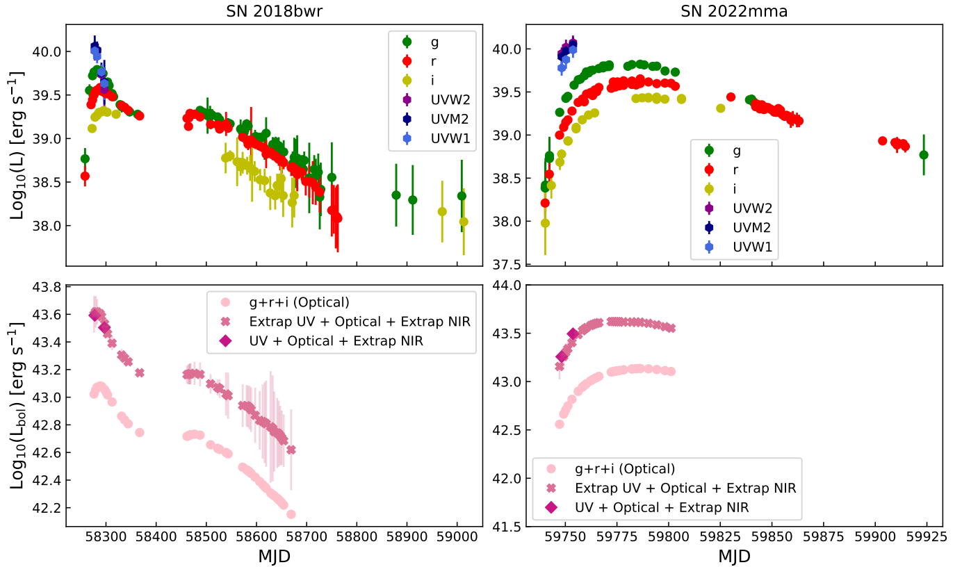
Fig. 10. Pseudo-bolometric light curves including UVOT observations. The top panels show the observed gri +UVOT light curves and the bottom panels the calculated pseudo-bolometric light curves for SN 2018bwr (left) and SN 2022mma (right).
