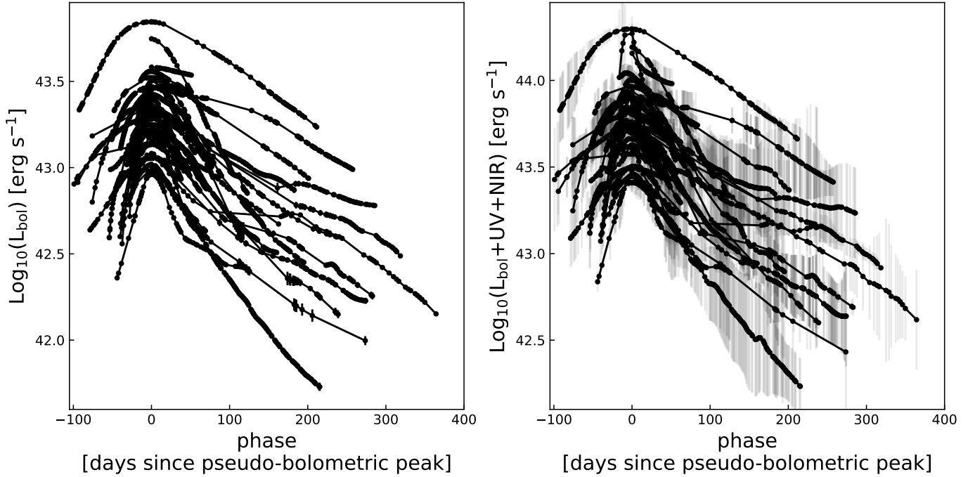
Fig. 9. Pseudo-bolometric light curves of the SLSN II sample. The left panel shows the results of integrating the observed SED considering the epochs for which we have all three gri photometric observations. The right panel shows the results of adding extrapolations to both the UV and NIR to the SED obtained from the gri photometric observations.
