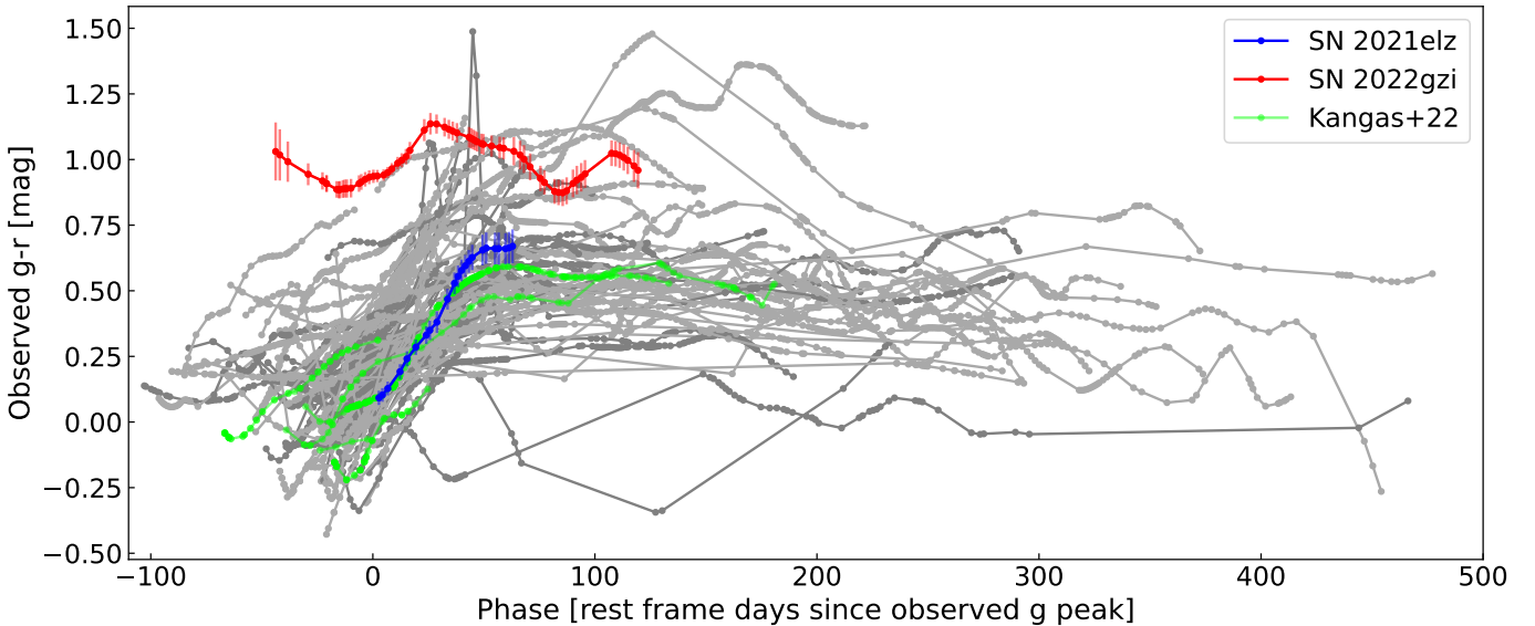
Fig. 7. Observed g - r colors with respect to rest frame days since g band peak. In dark gray, we show events at z < 0.17 and in light gray events at z \geq 0.17 . In red we highlight the event with the faintest rest frame peak absolute magnitude in g band, indicating that it may be suffering from considerable host extinction. In blue we highlight the event with the brightest rest frame peak absolute magnitude in g band, the color evolution of this SLSN II is consistent with the general trend of the sample. In lime we show the observed g - r colors of the events with z \leq 0.17 in the ZTF SLSN II sample presented by Kangas et al. (2022), see Sect. 5.1 for a discussion.
