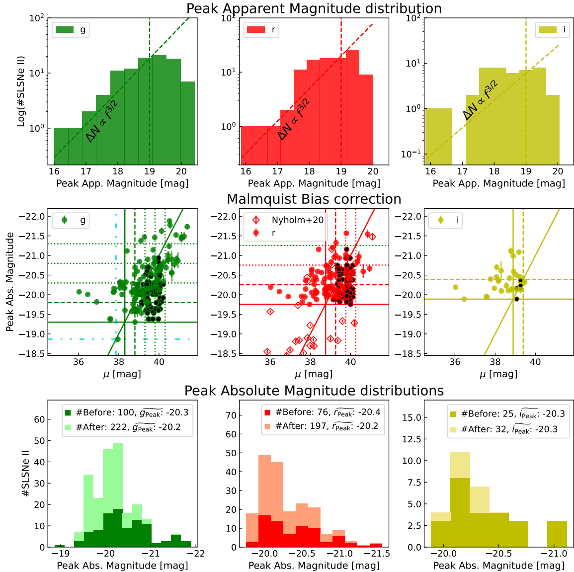
Fig. 12. Malmquist bias correction. The top row shows the peak apparent magnitude distribution of the observed sample in gri bands (left, middle, and right panels, respectively), the inclined dashed line shows the \Delta N \propto f^{3/2} relation, the vertical dashed line shows the integer magnitude closest to the last position at which the slope of this relation intersects the distribution. The second row shows the original rest frame peak absolute magnitude distribution with respect to the distance moduli in gri bands (left, middle, and right panels, respectively), together with the estimated distribution of missed events, presented as black dots. The solid horizontal lines indicate the faintest event of the distribution while the solid vertical lines indicate the corresponding distance modulus. The subsequent horizontal and vertical lines indicate 0.5 mag bins from the solid lines, respectively. The double dash-dotted turquoise lines in the first panel shows an event fainter than the one we consider for the analysis, we consider this event suffers from extinction and it is not considered. The third row shows the distribution of rest frame peak absolute magnitude in gri bands (left, middle, and right panels, respectively) before (dark colors) and after (light colors) applying the Malmquist bias correction.
