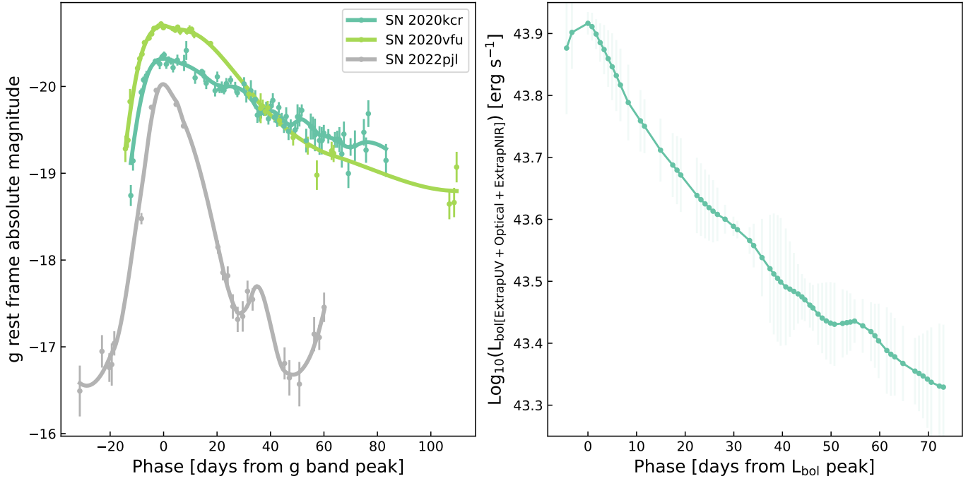
Fig. A.3. SLSNe II with t_{\text{rise},1/e} \leq 15 rest frame days in any of the gri photometric bands. Left panel: rest frame g band absolute magnitude with respect to rest frame days since g band peak. Right panel: pseudo-bolometric light curves of events with gri band observations.
