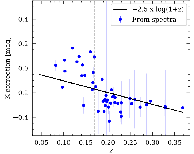
Fig. 2. K-correction approximation obtained as -2.5 \times \log(1+z) (black line), compared to full K-corrections obtained using SNooPy (blue dots). The inverse of the S/N of the spectrum considered to calculate full K-corrections is presented as associated error bars. The vertical dashed gray line indicates z = 0.17 , at which we switch from g to r band to calculate the correction.
