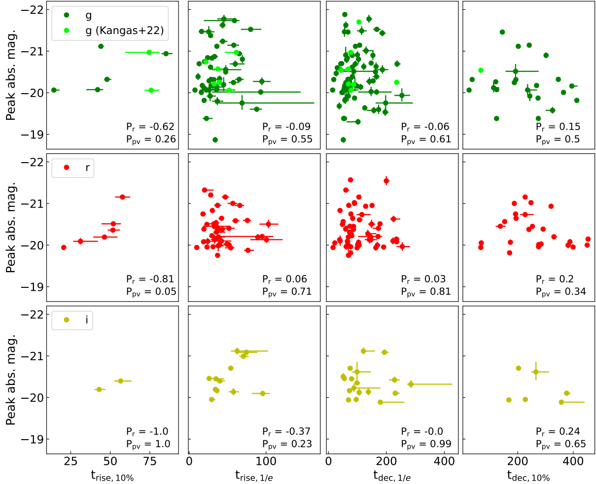
Fig. 5. Timescales versus peak absolute magnitudes. From top to bottom: gri band (respectively) rest frame peak absolute magnitude compared to t_{\text{rise},10\%} (first columns), t_{\text{rise},1/e} (second columns), t_{\text{dec},1/e} (third column) and t_{\text{dec},10\%} (last column). The corresponding Pearson's r parameter ( P_r ) and associated p value ( P_{pv} ) for each distribution is annotated in the bottom right of the corresponding panels, no significant correlation is found for these parameters. Lime dots in the first row show the corresponding parameter distribution of the ZTF SLSN II sample presented by Kangas et al. (2022), see Sect. 5.1 for a discussion. These additional events are not included in the correlation analysis.
