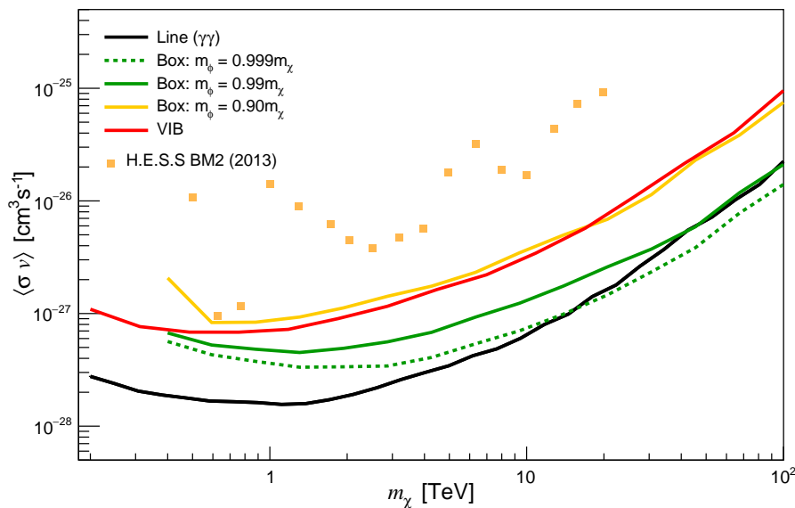
Figure 9. Expected median 95% C.L. exclusion limits, from GC observations, for the spectral shapes shown in figure 2: VIB (red), a relatively wide box with m_\phi = 0.9m_\chi (orange) and a narrow box with m_\phi = 0.99m_\chi (green). For comparison, we also show the case of an extremely narrow box with m_\phi = 0.999m_\chi (dotted green) and the result for a monochromatic line signal (black, same as in figure 6). Note that the analysis windows for the narrow box spectra are centred around E = m_\chi/2 , the wide box spectrum is centred at the upper edge E = (m_\chi + \Delta E)/2 , while those for VIB and line spectra are centred around E = m_\chi ; as a consequence, the lowest mass points that we include in our analysis are given by m_\chi = 0.4 TeV and m_\chi = 0.2 TeV, respectively. We also indicate previous 95% C.L. limits obtained by H.E.S.S. [20] for a signal shape model (BM2 from ref. [17]) that closely resembles the VIB signal studied here, rescaled to the DM profile adopted in this analysis for the sake of comparison (see footnote 10 for further details).
