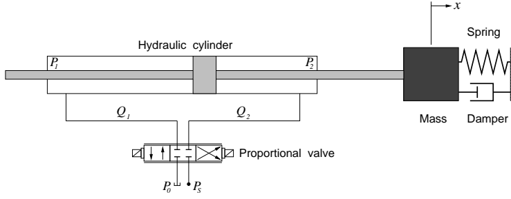
Fig. 1 Schematic diagram of the electro-hydraulic servo-system.
