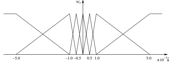
Fig. 3 Adopted fuzzy membership functions.
