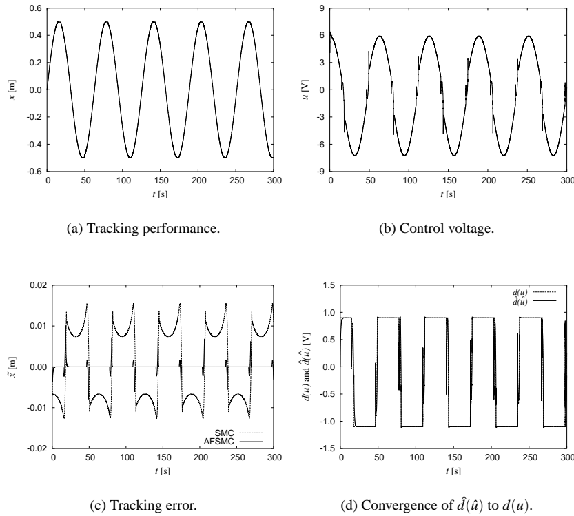
Fig. 4 Tracking performance with unknown dead-band and well known model parameters.
