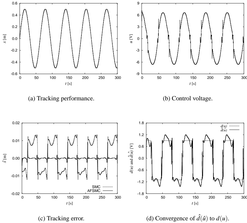
Fig. 5 Tracking performance with unknown dead-zone and uncertain model parameters.
