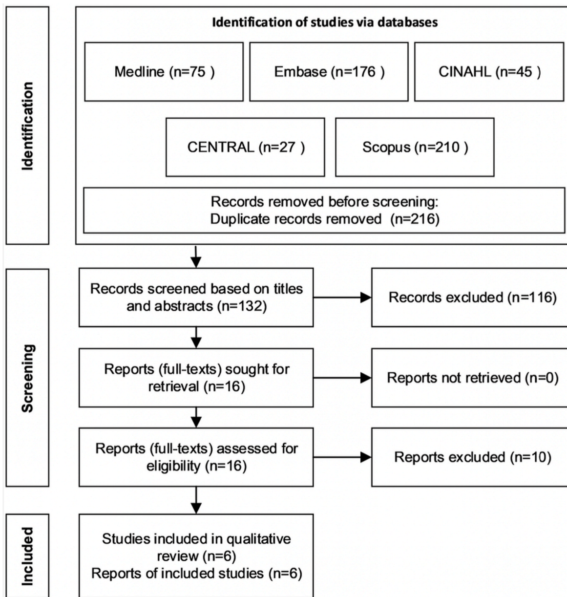
Fig. 1. Selection strategy.
