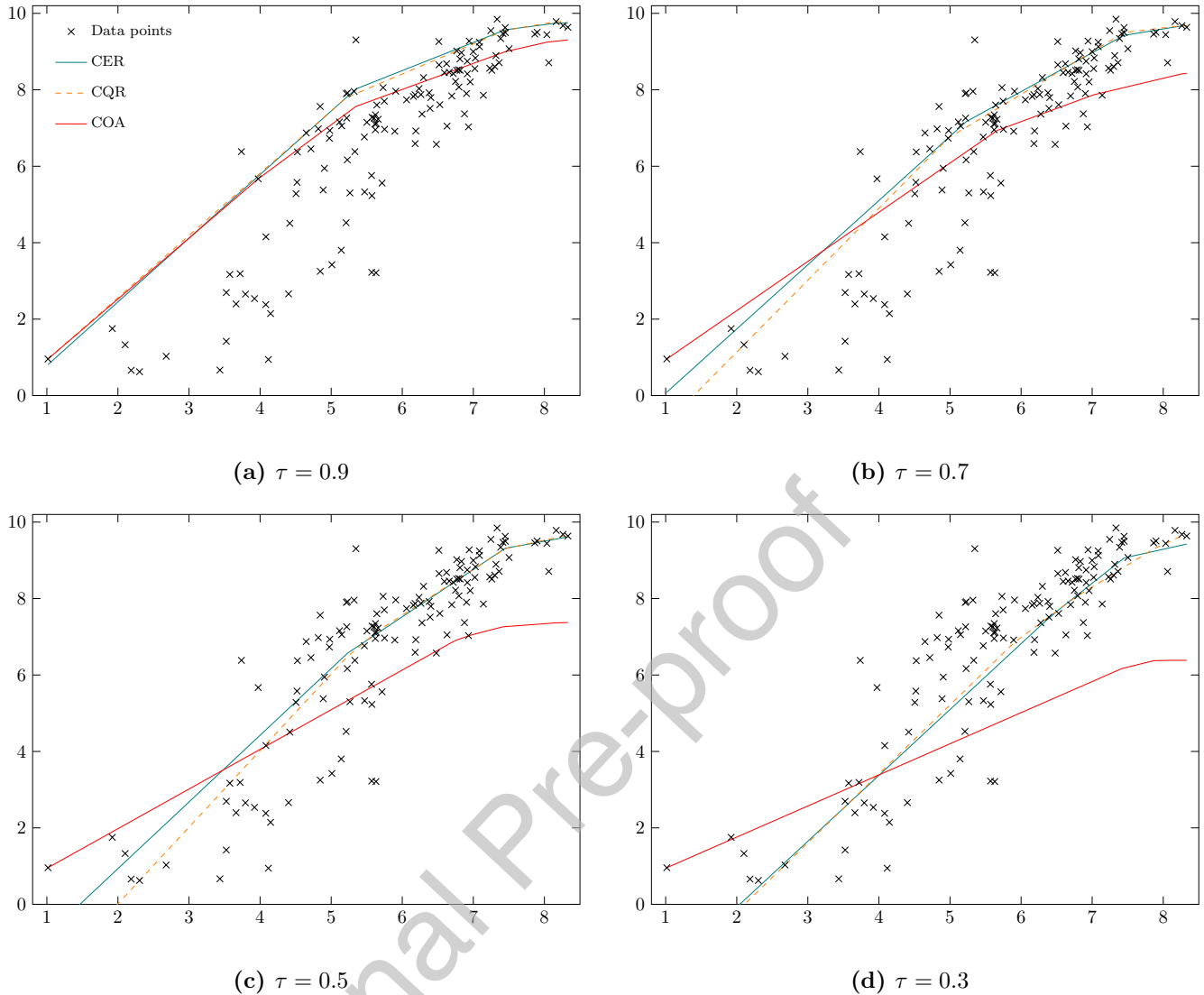
Fig. 6. Illustration of the estimated convexified order- \alpha , CQR, and CER functions. X-axis: \ln(C) , Y-axis: \ln(Q) .
