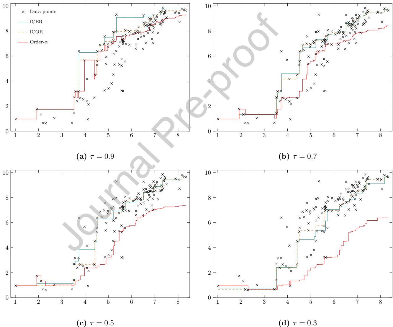
Fig. 5. Illustration of the estimated order- \alpha , isotonic CQR, and isotonic CER functions. X-axis: \ln(C) , Y-axis: \ln(Q) .
