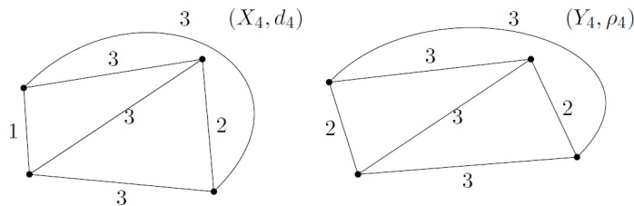
Fig. 1. (X_4, d_4) and (Y_4, \rho_4) are not US -spaces by Theorem 2.14
