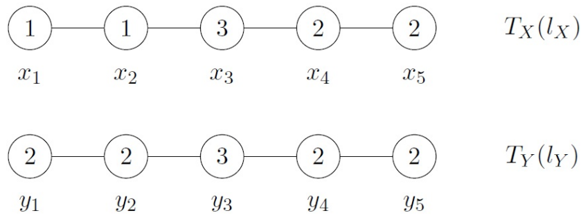
Fig. 3. The ultrametric space (V(T_X), d_{l_X}) contains the four-point subspace \{x_1, x_2, x_4, x_5\} which is isometric to (X_4, d_4) . Similarly, (V(T_Y), d_{l_Y}) contains the subspace \{y_1, y_2, y_4, y_5\} which is isometric to (Y_4, \rho_4)
