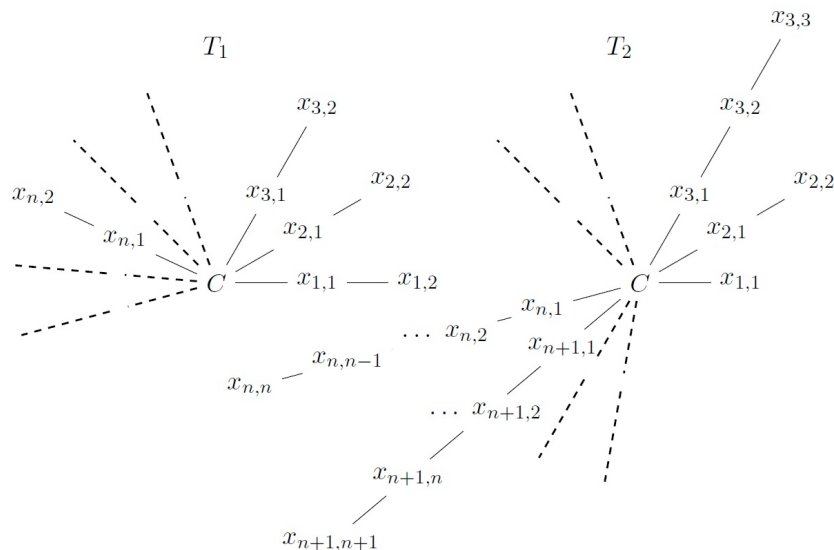
Fig. 4. Trees T_1 and T_2 are starlike and rayless
