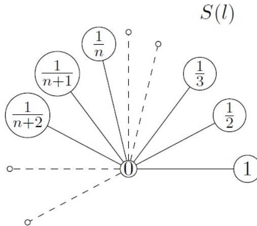
Fig. 2. The unique point x_0 satisfying (6) for all x, y \in Y which satisfy (7), is the center of the labeled star graph S(l)
