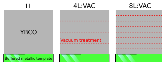
Fig. 1. The schematic diagram of the multilayer structures, where 4 \times 500 (4L:VAC) and 8 \times 250 (8L:VAC) pulses of YBCO were deposited with 2 min vacuum treatment between the layers. The film structures were deposited on the metallic hastelloy C276 template with IBAD-MgO based buffer layers and the YBCO single layer film of 2000 pulses (1L) is prepared for comparison. The total thickness of 1L, 4L:VAC and 8L:VAC films is \approx 380 nm.
