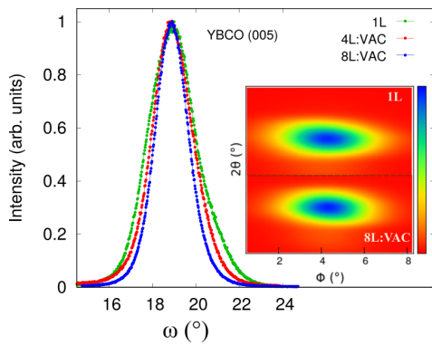
Fig. 2. The normalized XRD rocking curves ( \omega -scans) of the YBCO (005) peaks measured from the YBCO multilayers (the main panel). In the inset, the XRD (102) peaks as functions of 2\theta and relative \phi are given for the samples 1L and 8L:VAC.
