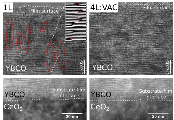
Fig. 3. Cross-sectional HRTEM images of samples 1L and 4L:VAC, where the upward direction corresponds to YBCO c -axis. The bottom images in both 1L and 4L:VAC are taken from the interface of top buffer layer \text{CeO}_2 , while the images on the top are from the surface layer of the films. The red markings on the image of film 1L indicate the edge dislocations collectively positioned along the YBCO c -axis, as also shown in the inverse FFT image on the top right corner.
