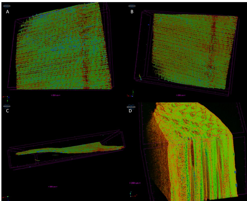
Figure 9. CT-scans of bamboo PA. Leaf: A) upper surface, B) lower surface, C) cross-section and D) stem. PA. Blue areas represent areas of high density phytoliths. Bar = 250 \mu\text{m} .
