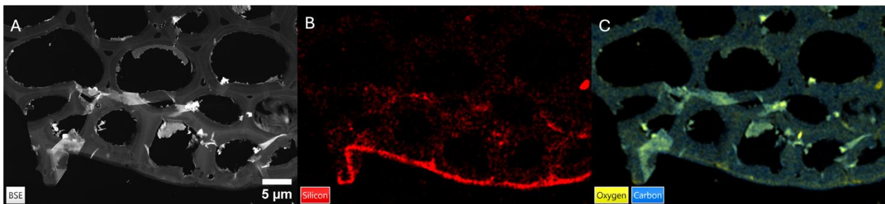
Figure 6. A BSE (backscattered electrons) micrographs of cortex of bamboo. EDS micrographs from same area than Figure 5 A. B showing presence of silicon on the cortex. C showing oxygen and carbon location on bamboo cortex.
