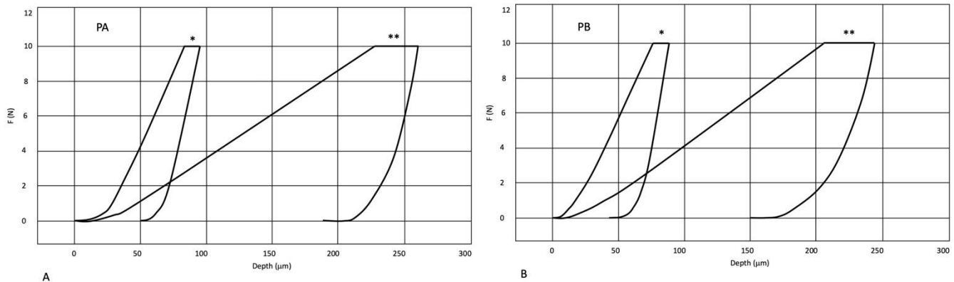
Figure 8. Load-displacement curve of surface microhardness. A) Bamboo PA; B) bamboo PB. * refers indentation of outer cortex and ** inner part of the stem.
