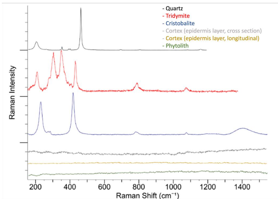
Figure 7. RAMAN spectra of reference of quartz, tridymite and cristobalite showing typical Raman shift for the crystal structure. Gray and yellow lines are showing amorphous structure of precipitation of silica in bamboo cortex and underlying epidermis layer of the stem. Green line shows amorphous structure of phytolith from leaf.
