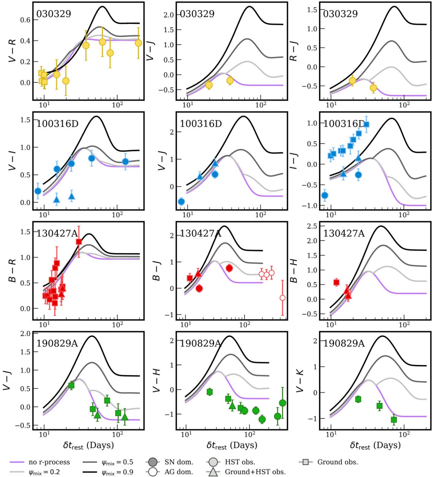
Figure 4. Sorted colors of the four GRB-SNe in our sample vs. rest-frame time compared to the best-fit models from Barnes & Metzger (2022; Figure 3 and Section 4) with fixed r -process mass ( M_{\text{rp}} = 0.03 ) and varying values of \psi_{\text{mix}} (lines). We also plot models without r -process enrichment in purple. Afterglow-dominated observations are shown as open symbols, and measurements dominated by SN emission are shown as filled symbols. Though color measurements between filters vary, none of our late-time measurements favor high values of \psi_{\text{mix}} . Many measurements, particularly those that extend to late times, are unable to distinguish between models with \psi_{\text{mix}} \lesssim 0.2 and those with no r -process. GRB 190829A is, in the best-sampled V-H filters, bluer than the unenriched models.
