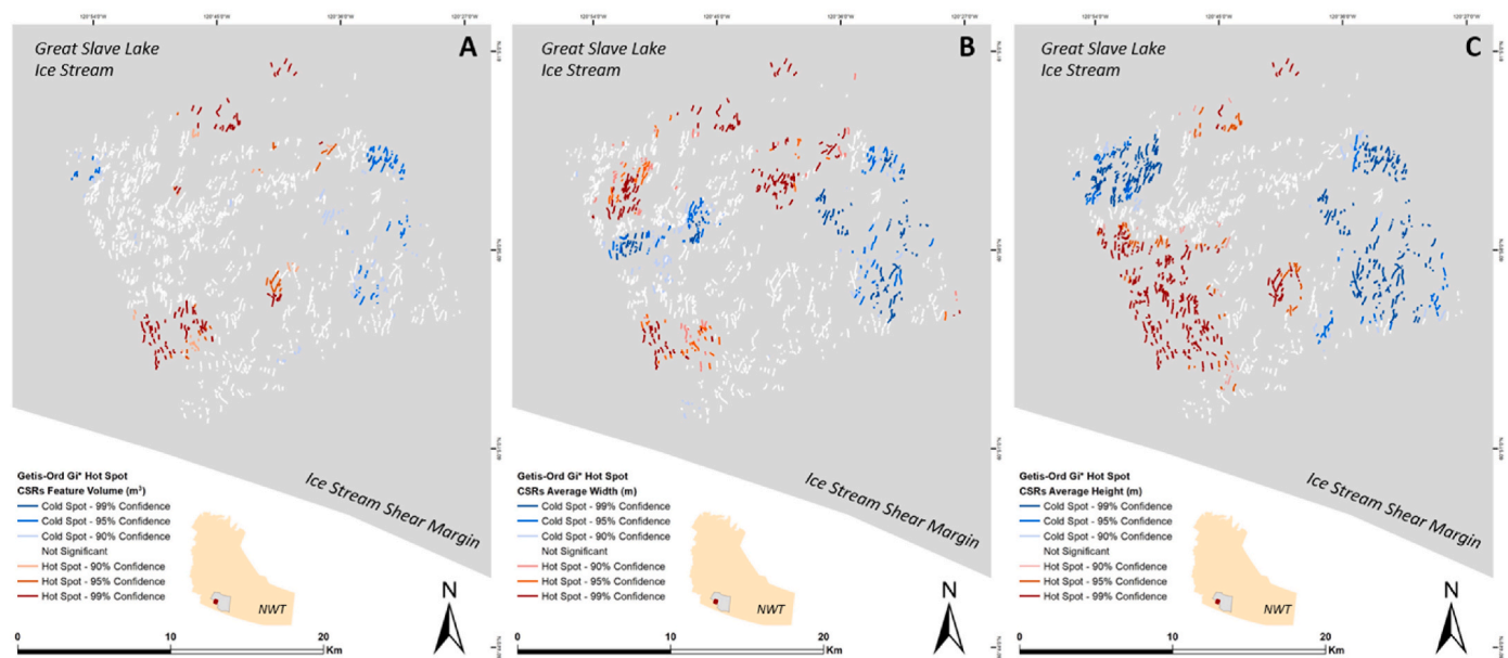
Fig. 11. Results of 'getis-ord gi*' hot spot analysis'. A) CSR total feature volume; B) CSR average feature width; and C) CSR average feature height.
