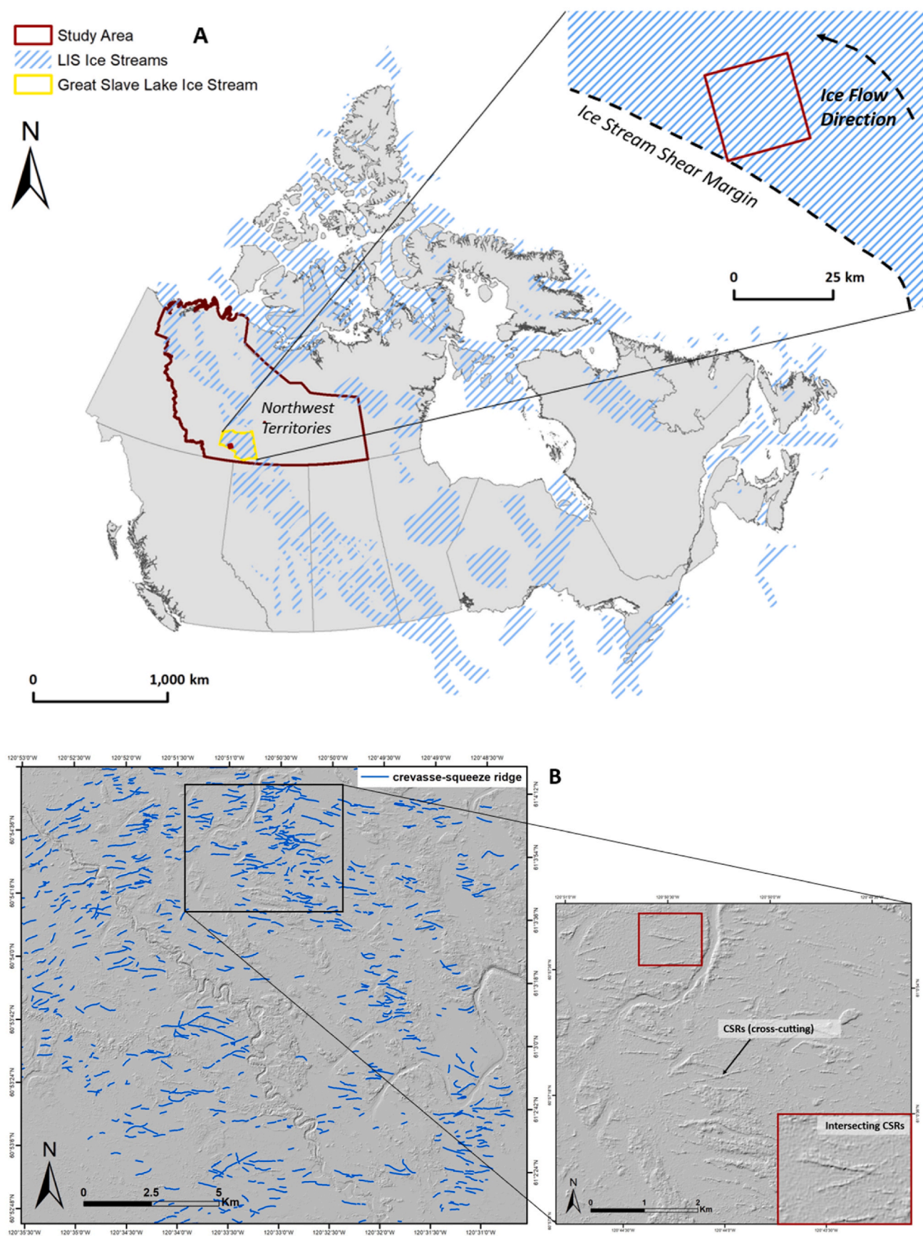
Fig. 5. A) Study area selected for CSR data collection. Location: Great Slave Lake palaeo-ice stream, Northwest Territories, Canada [ice stream data source: Margold et al., 2015 ]. Location map shows the study area situated inside of the shear margin of the Great Slave Lake ice stream. B) Hillshaded DEM showing mapping extent of CSRs at study area. The imagery shows CSRs arranged in a linear, sometimes cross-cutting swarm. [DEM source: ArcticDEM – Porter et al., 2018 ].
