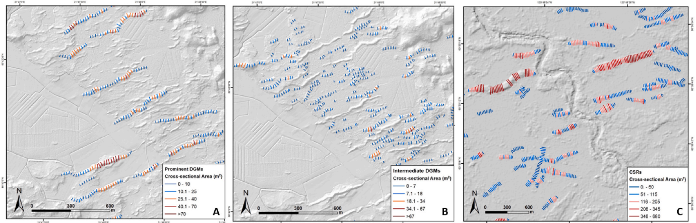
Fig. 9. Transect morphometry visualisation showing transects generated at 20 m intervals for each identified landform group: A) prominent DGMs, B) intermediate DGMs and C) CSRs. The ‘cross-sectional area’ calculated along each transect are shown and colour-graded to represent high (red) – low (blue) values. Each dataset were categorised using the ArcGIS automated natural breaks (Jenks) method. [DEM sources: A & B: ©National Land Survey of Finland, LiDAR digital elevation model, February 2023; C: ArcticDEM - Porter et al., 2018].
