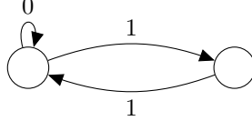
Figure 3: The graph of the even shift.
