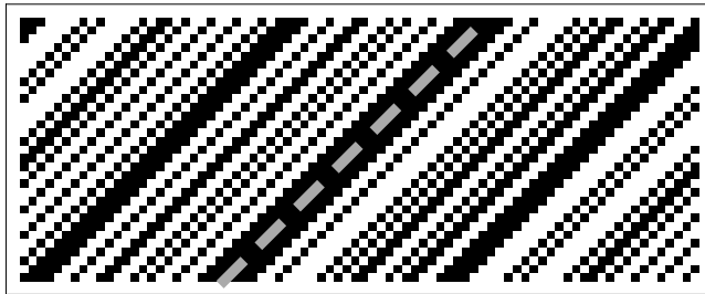
Figure 2: A space-time diagram of the binary shift map \sigma . White and black squares correspond to digits 0 and 1 respectively. The dashed line shows an almost equicontinuous direction.
