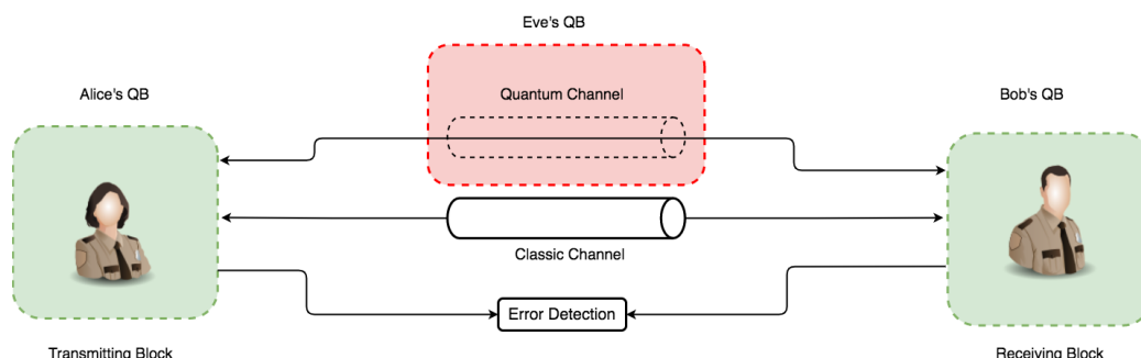
Figure 3. This is a figure representing the base overview of the simulation concept for subsequent simulation iterations.
