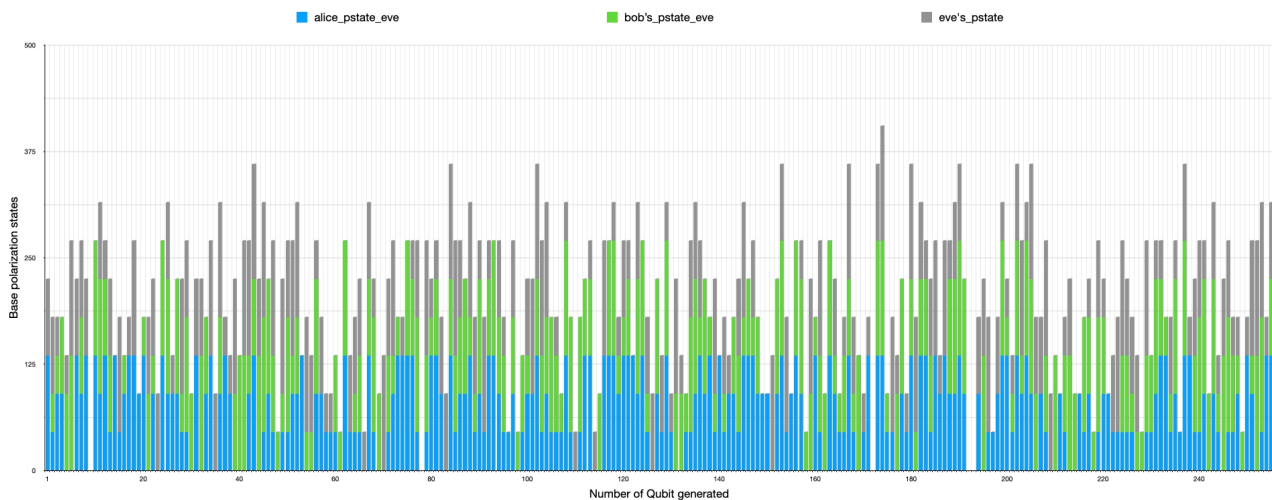
Figure 15. A 2D stacked bar chart with the sender's, receiver's, and Eve's polarization states in the second simulation instance (with the presence of Eve), indicating the chosen and measured qubit randomness.
