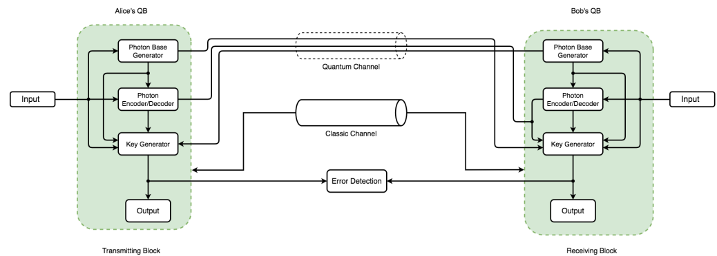
Figure 5. Simulation model design used for simulating an instance without the presence of eavesdropping (Eve's quantum block).
