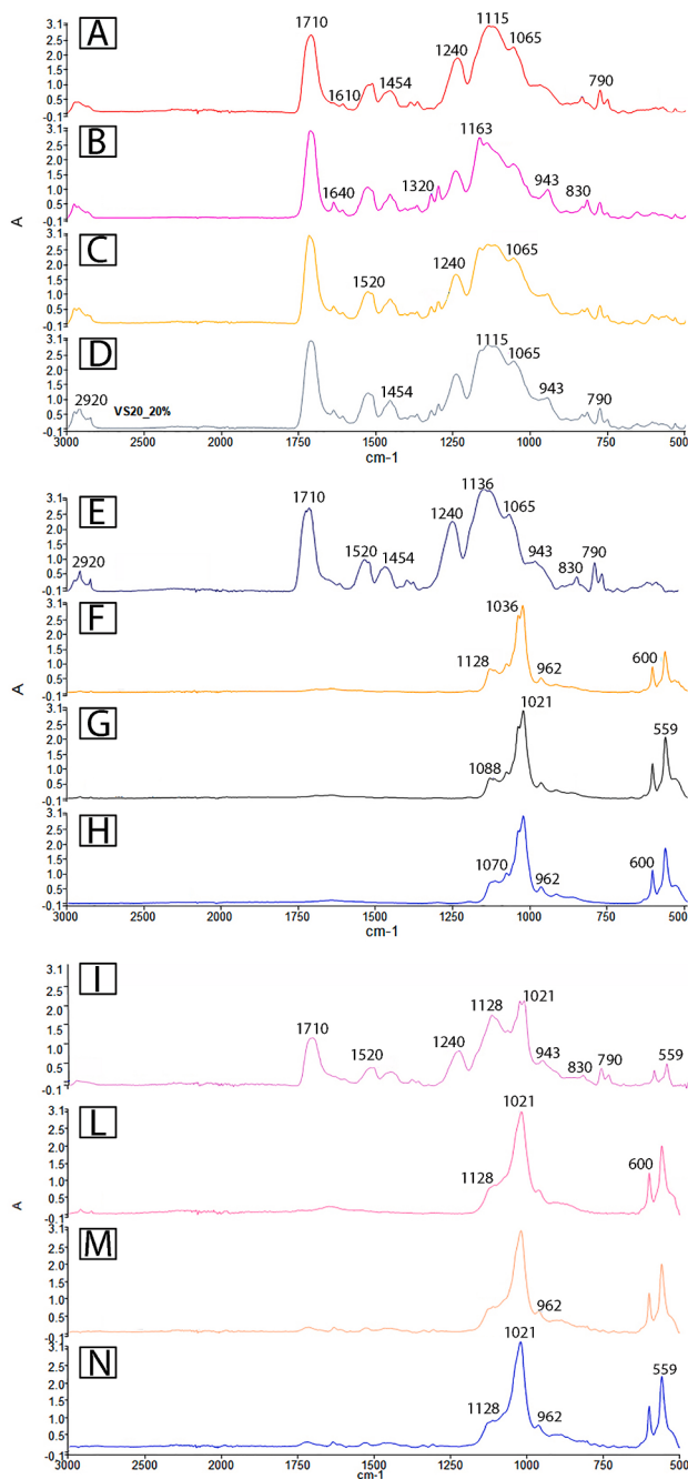
Fig. 1. Infrared spectra of reference and experimental composites with FCDC filler. (A) Spectrum of the control composite without FCDC filler at baseline, showing characteristic peaks of organic methacrylate monomers. (B) VS10-5 %, (C) VS10-10 %, (D) VS20-20 %, with the additional peak at 1136\text{ cm}^{-1} associated with the stretching modes of the pyrophosphate anion ( \text{P}_2\text{O}_7^{4-} ). (E) Control composite without FCDC filler after 30 days in simulated body fluid (SBF), exhibiting spectra similar to baseline. (F) VS10-5 % after 15 days, (G) VS10-10 % after 7 days, and (H) VS10-20 % after 15 days of SBF storage, showing all the PO stretching peaks of hydroxyapatite. (I) VS20-5 % without apatite formation after 15 days in SBF, while (L) VS20-5 % displays clear apatite formation on the surface after 30 days. The only material to exhibit clear PO stretching peaks of hydroxyapatite after 7 days is the composite (M) VS20-10 %, whereas composite (N) VS20-20 % requires 15 days of SBF storage to show a distinct formation of apatite on the surface.
