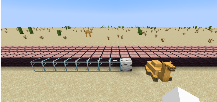
FIGURE 1. The group \mathbb{Z}^3 visualized in Minecraft 1.21.1 [24], with the first axis pointing right, the second axis forward, and the third axis upward. The inductive interval with axis intervals ([-8, -1], [1, 5], [-64, -1]) is filled with blocks: a block of birch marks the origin, glass is used to fill on the first axis, cherry tree trunks on the second, and desert sand on the last. Plants and camels appear organically and serve no mathematical purpose. The interval [-64, -1] denotes the depth of the layer of sand, which is not visible in the picture (colour online).
