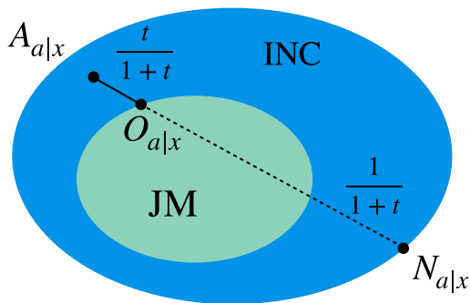
FIG. 3. Illustration of the incompatibility robustness. JM, compatible sets; INC, incompatible sets. The POVMs \{A_{a|x}\} are mixed with arbitrary noise POVMs \{N_{a|x}\} such that their mixture is compatible. The incompatibility robustness is the smallest t that realizes such a decomposition; cf. Eq. (25).
