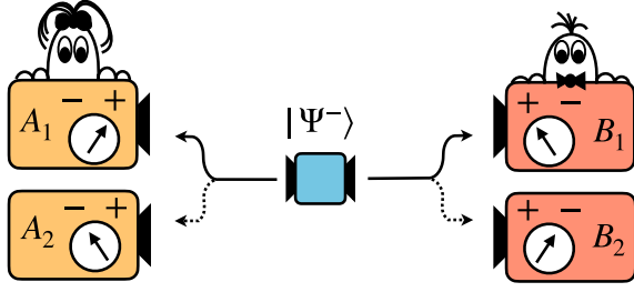
FIG. 5. Schematic of the Bell scenario. A source distributes two particles to two parties named Alice and Bob. They perform measurements on it, and the questions arises as to whether or not the observed probability distribution can be described by a local hidden variable model.
