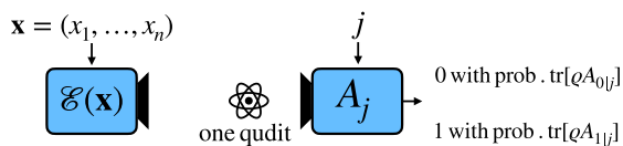
FIG. 7. Schematic of quantum random access codes. A sender holds n bits of information \mathbf{x} and encodes it into a single qudit via the quantum channel \mathcal{E}(\mathbf{x}) . The receiver wants to recover a random bit x_j from \mathbf{x} by performing a measurement \{A_{x_j|j}\} on the qudit.
