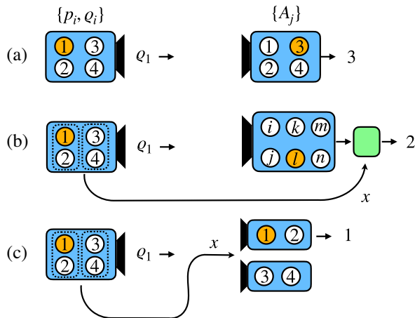
FIG. 6. Quantum state discrimination in different scenarios. (a) In minimum-error state discrimination the task is to guess the correct input label of the state with high probability. (b) In state discrimination with postinformation, the label x is revealed after the measurement. Here the additional information can be used only to postprocess the classical measurement result. (c) In state discrimination with prior information, the partition x of the label is received before the state, and hence a different measurement can be tailored to each subset x of the labels. Adapted from Carmeli, Heinosaari, and Toigo, 2018.
