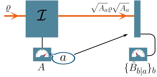
FIG. 8. Illustration for a joint measurement (a parent measurement) for the target POVMs A and B . As long as A and B are jointly measurable, by first performing the Lüders measurement of A and then, conditioned by the outcome a obtained in the A measurement, measuring a conditional POVM \{\tilde{B}_{b|a}\}_b after the A measurement, this sequential scheme realizes a joint measurement of A and B .
