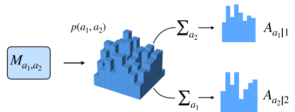
FIG. 1. Marginal form joint measurement of two POVMs. The data of the joint measurement are presented as a grid from which marginalization gives the data of the original pair of measurements.
