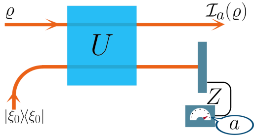
FIG. 9. The “auxiliary” Naimark dilation has a particular form that enables the following physical interpretation of an instrument \mathcal{I} measuring the target POVM A (Ozawa, 1984). The system state is coupled with a probe (the auxiliary system in the dilation) in the initial state |\xi_0\rangle \langle \xi_0| . A unitary evolution mediated by the unitary U then takes place followed by a sharp pointer measurement Z of the probe, after which the probe is detached from the system.
