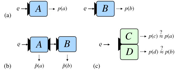
FIG. 2. Schematic view of measurement uncertainty relations. (a) For any quantum state \rho the measurement A yields results with a probability distribution p(a) ; similarly, B delivers a distribution p(b) . (b) A possible way to study the disturbance of B through A is to measure in sequence and compare the distributions \tilde{p}(a) and \tilde{p}(b) to p(a) and p(b) . The reverse order of measurements can also be considered. (c) Since the measurements in (b) give probability distributions other than in (a), they can be described by different POVMs C and D . But C and D are then jointly measurable by construction. The question arises: What is the best approximation of A and B by two jointly measurable POVMs C and D ?
