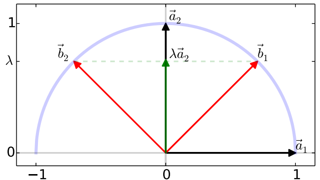
FIG. 4. An equally weighted coin toss between the auxiliary elements B_{+|1}(\lambda, \lambda) and B_{+|2}(\lambda, \lambda) with \lambda = 1/\sqrt{2} results in an effect with the Bloch vector \lambda\vec{a}_2 = \lambda(0, 0, 1) = (0, 0, 1/\sqrt{2}) . Here \vec{b}_1 and \vec{b}_2 are the Bloch vectors of B_{+|1}(\lambda, \lambda) and B_{+|2}(\lambda, \lambda) . The vectors \vec{a}_1 and \vec{a}_2 represent the directions of the original measurements.
