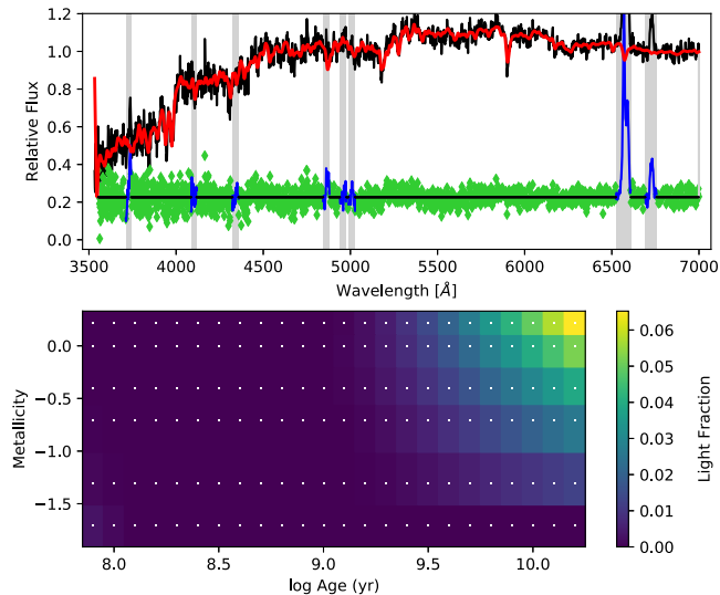
Figure 11. PPF modelling of the spectrum of neighbouring galaxy SDSS J232323.37 + 104101.7.
