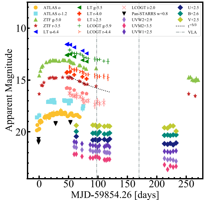
Figure 2. AT2022wtn UV/optical light curve. The optical data are host-subtracted. Magnitudes are reported in the AB system and are not corrected for foreground extinction. Vertical dot–dashed grey lines show the location of the VLA detection. We show the t^{-5/3} decline with a dotted line overplotted on the ZTF r' points.
