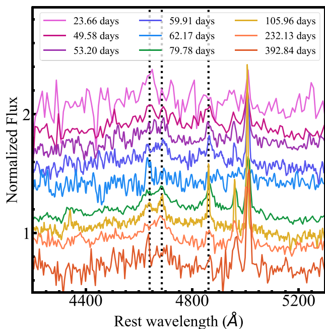
Figure 6. AT2022wtn spectral evolution in the N III + He II \lambda 4686 wavelength region. Starting from 59.91 d from the transient discovery the appearance of two separate components ascribable to the N III \lambda 4640 and He II \lambda 4686 is clearly visible. Dotted vertical lines indicate the N III \lambda 4640 , He II \lambda 4686 , and H \beta position.
