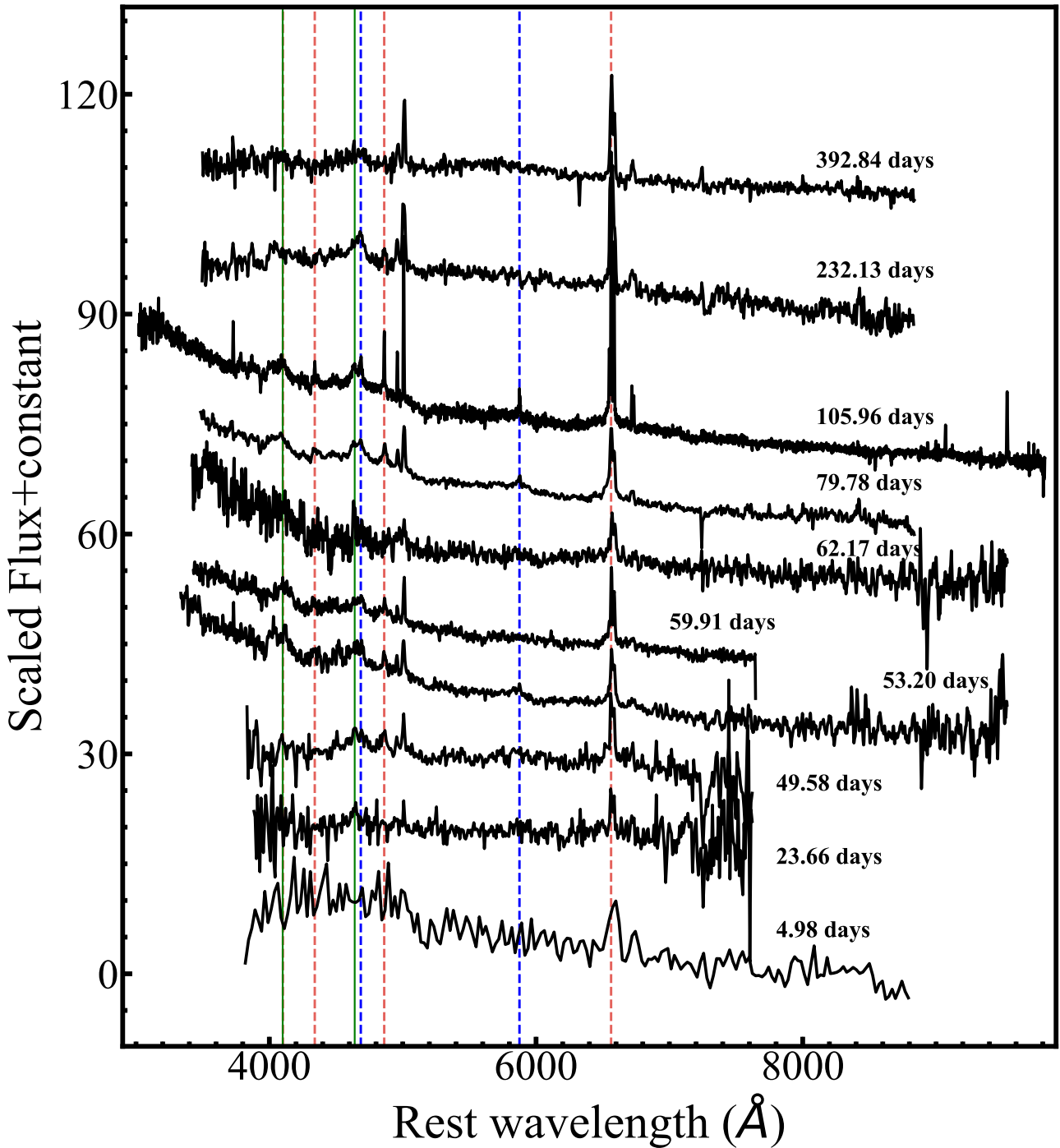
Figure A1. Sequence of AT2022wtn rest-frame optical spectra corrected for galactic extinction. Days from the transient discovery are shown. The position of the main TDE emission lines are indicated with coloured vertical lines: Hydrogen with red dashed lines, Helium with blue dashed lines, and Bowen lines with green solid lines.
