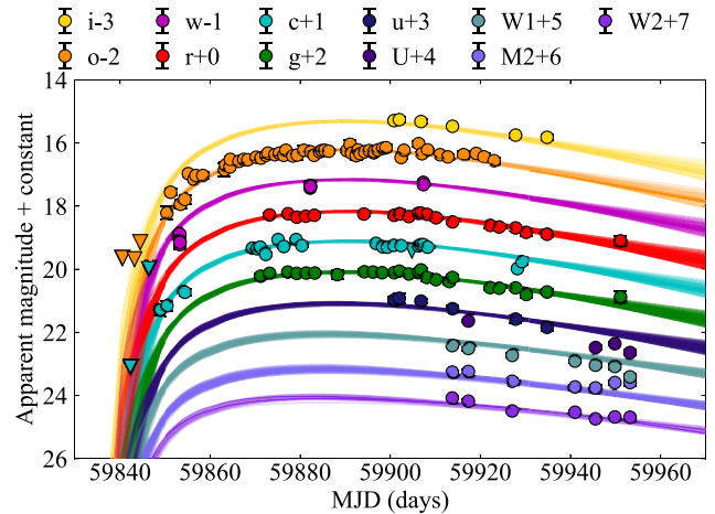
Figure 12. MOSFIT fit of the AT 2022wtn multicolour light curves.
