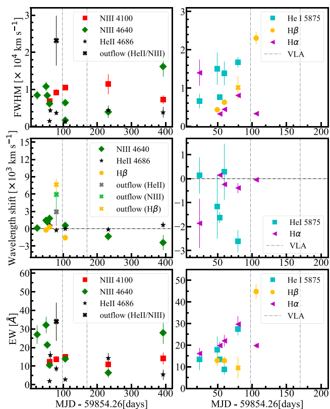
Figure 7. Upper panels: FWHM evolution of the broad components detected in the AT2022wtn spectral sequence for the [N III] \lambda \lambda 4100 and 4640, and the He II \lambda 4686 ; the H \beta , He I \lambda 5875 ; and H \alpha (left and right panels, respectively). Middle panels: evolution of the central wavelength shift for the broad and intermediate components detected in the AT2022wtn spectral sequence for the [N III] \lambda 4640 , He II \lambda 4686 , H \beta , He I \lambda 5875 ; and H \alpha (left and right panels, respectively). Bottom panels: EW evolution of the broad components detected in the AT2022wtn spectral sequence for the [N III] \lambda \lambda 4100 and 4640 and the He II \lambda 4686 ; H \beta , He I \lambda 5875 ; and H \alpha (left and right panels, respectively). The coloured cross markers indicate the possible outflows components. The dashed grey vertical line shows the location of the VLA detection.
