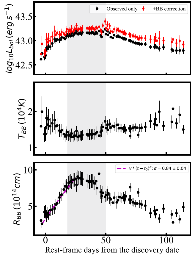
Figure 3. Superbol output showing the pseudo-bolometric light curve (upper panel), the T_{BB} (central panel), and the R_{BB} (bottom panel) time evolution. The input magnitudes are host-subtracted and have been corrected for reddening. The data are plotted with a bin of 1 d. Grey area indicate the duration of the maximum luminosity plateau phase. The magenta dashed line in the bottom panel shows the best fit for the R_{BB} rising phase.
