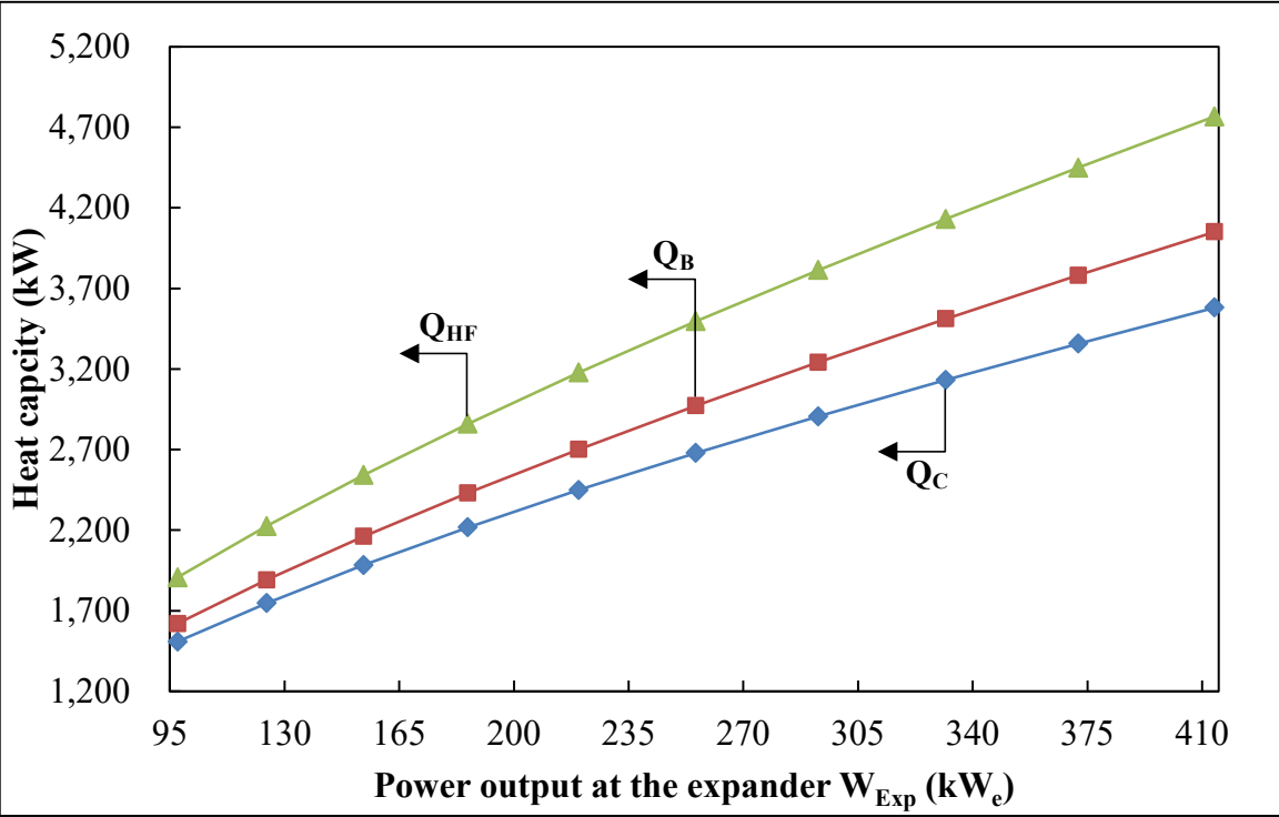
Fig. 2. Heat capacity of the hot water, boiler, and condenser in the ORC system.
