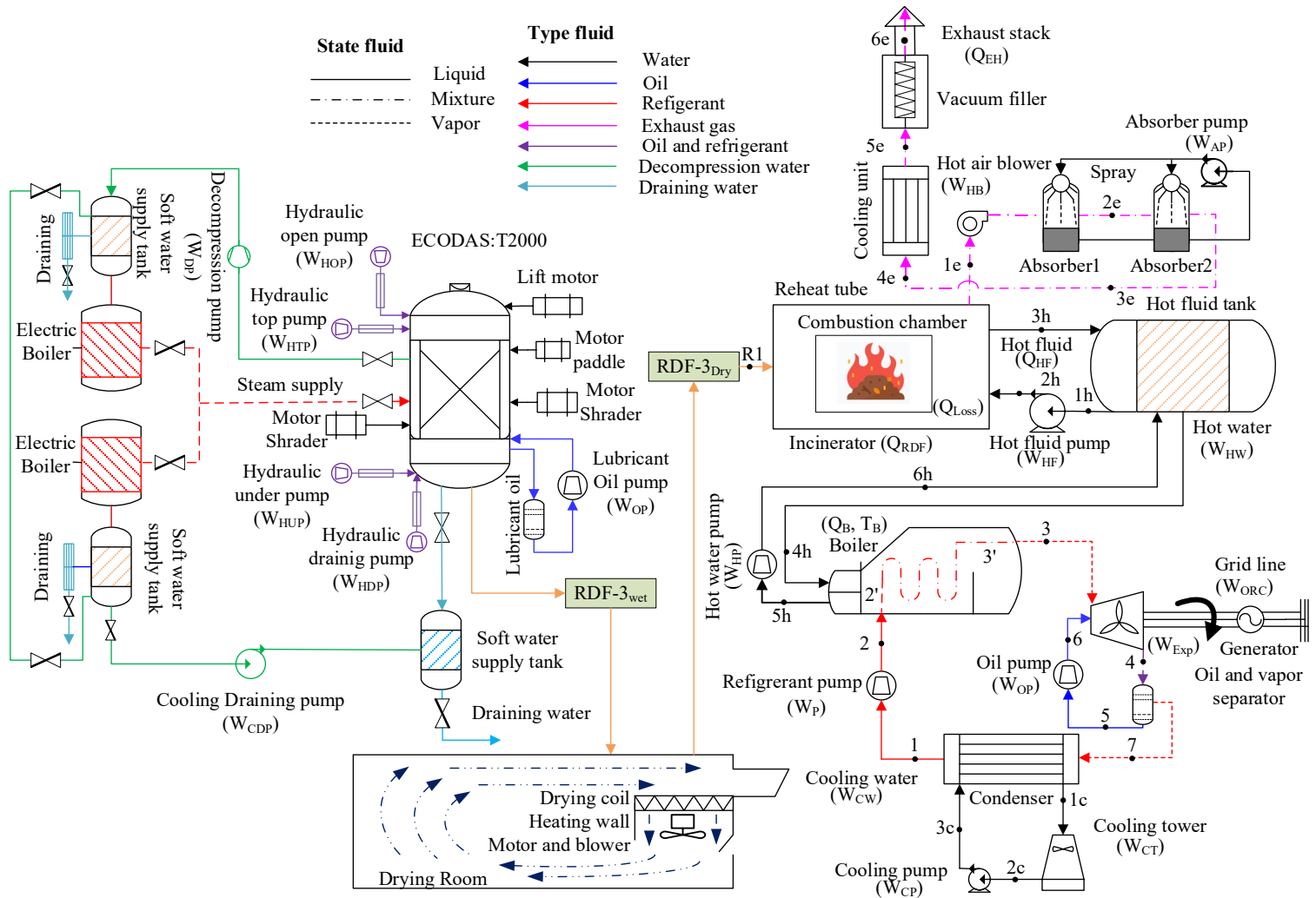
Fig. 1. Infectious medical waste treatment and Organic Rankine Cycle system.
