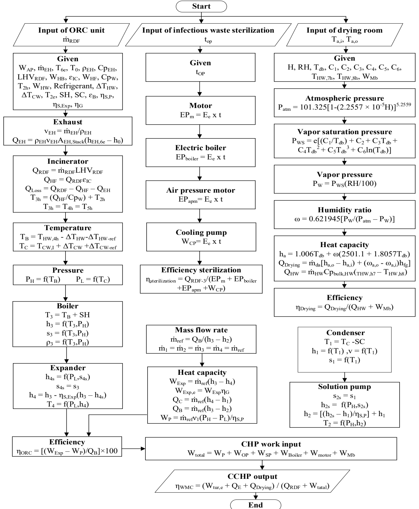
Fig. 2. Waste management center, incinerator, and ORC performance
