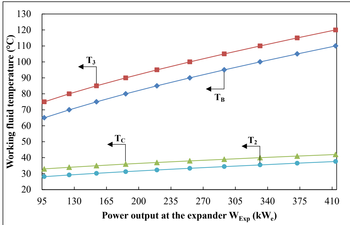
Fig. 4. Working fluid temperature in the ORC system.
