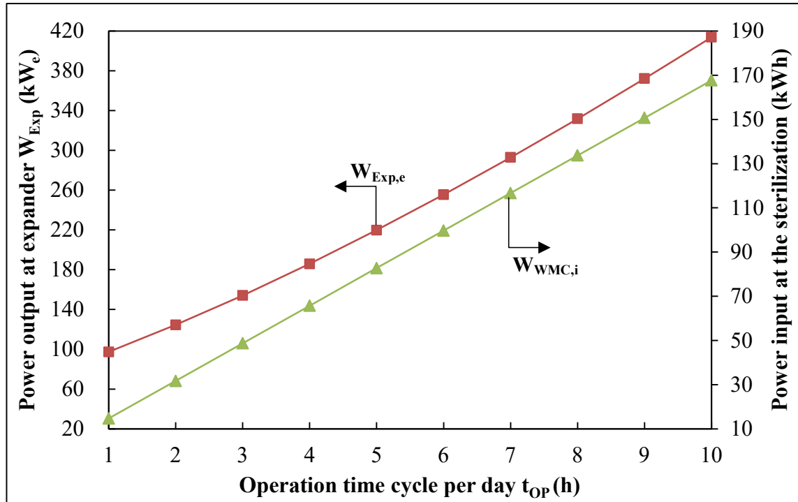
Fig. 7. Comparison of the input power for sterilization and the power output of the ORC
