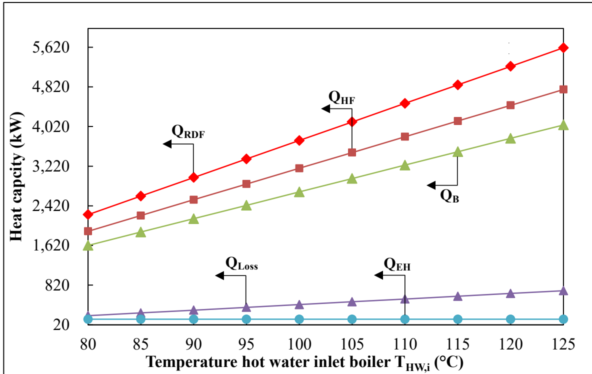
Fig. 1. Heat capacity of the incinerator and ORC system.
