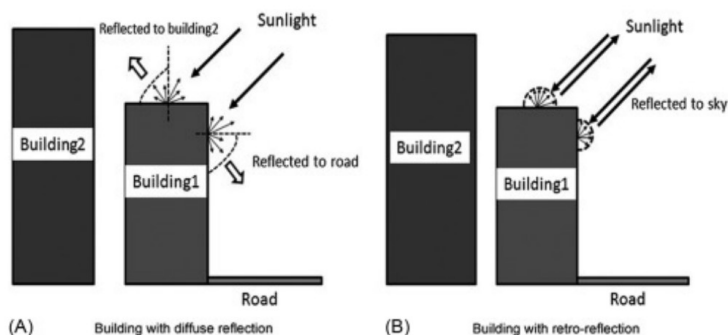
Figure5: Difference between diffuse reflection and retro-reflection (Pérez, Castro, Melo, & Xamán, 2017)
