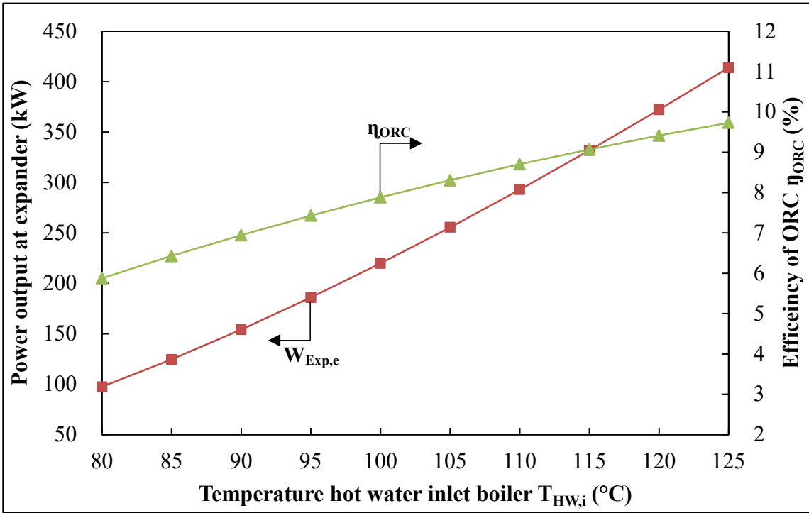
Fig. 6. Energy efficiency of the ORC system.
