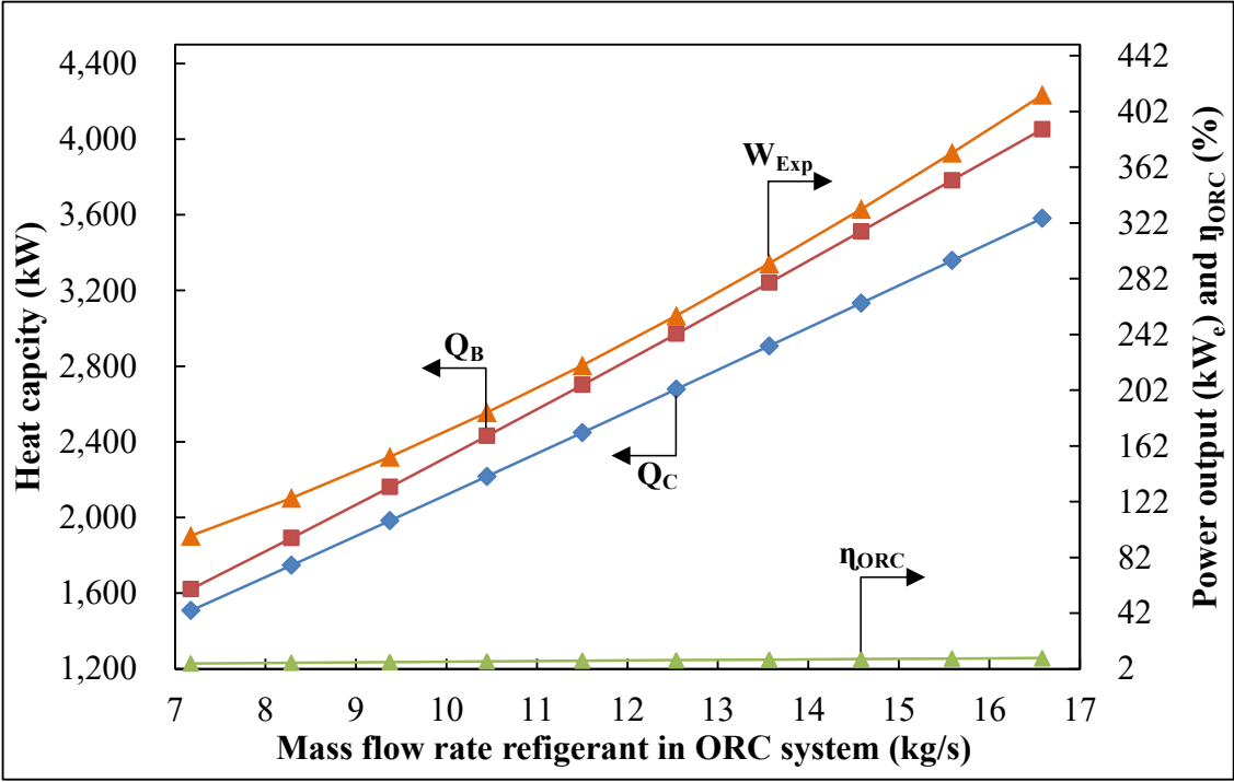
Fig. 5. The power output at the expander in heat capacity impact.
