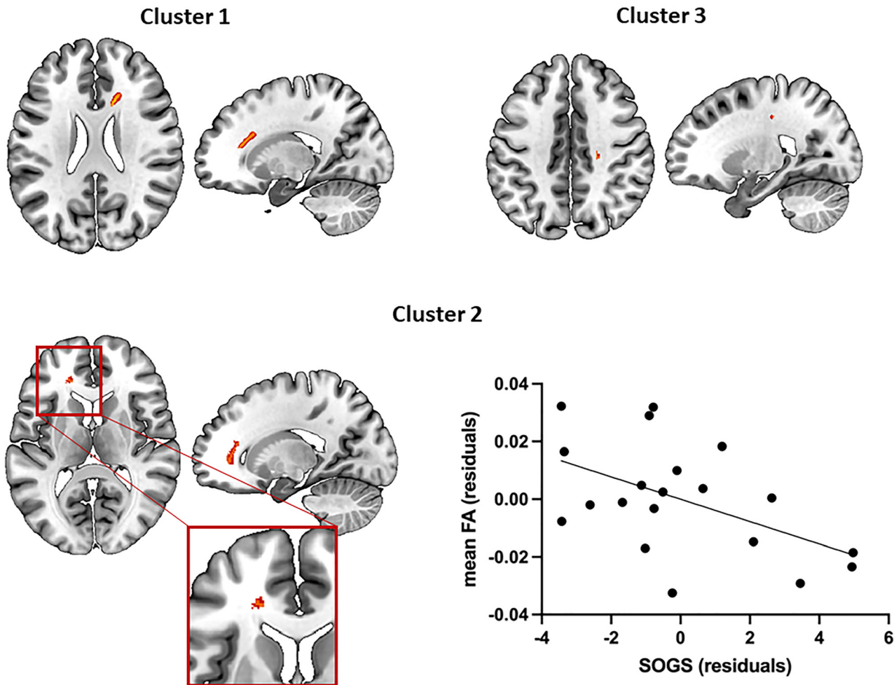
Fig. 1. FA differences between groups and correlation with SOGS scores
