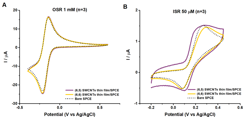
Fig. 5 Average of three cyclic voltammograms of SWCNTs thin film/SPCEs with a scan rate of 100 \text{ mV s}^{-1} in (A) \text{Ru}(\text{NH}_3)_6^{3+/2+} 1 mM in 1 M KCl and (B) DA 50 \mu\text{M} in PBS.
