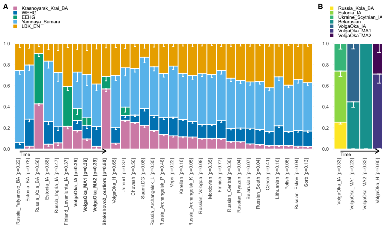
Figure 3. Results from qpAdm analyses
