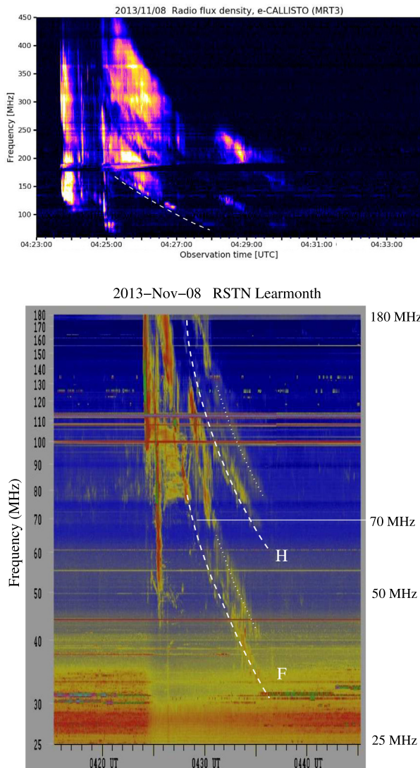
Fig. 7. Tracing the type II lanes in the e-CALLISTO MRT3 dynamic spectrum in the frequency range of 450–50 MHz (top) and in the RSTN Learmonth spectrum at 180–25 MHz (bottom). The fundamental (F) and harmonic (H) lanes are band-split (indicated with dashed and dotted lines in the Learmonth spectrum, respectively). We used the fundamental, lower band-split lane in the height calculations. The times and heights are listed in Table 2 and they are shown in Figs. 2 and 9. The type II emission was preceded by type III bursts, which makes it difficult to define the exact type II burst start time.
