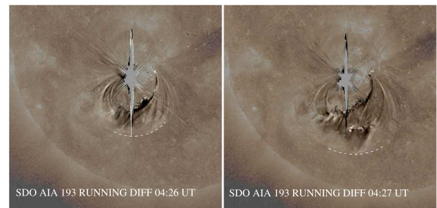
Fig. 3. SDO/AIA 193 Å difference images that show the evolution of the EUV wave that followed the GOES X1.1 class flare located at S14E15.
