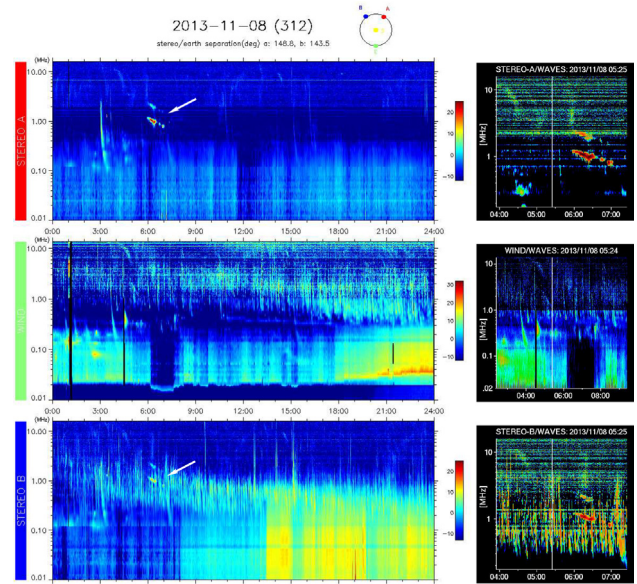
Fig. 8. STEREO A/SWAVES (location A in red), Wind/WAVES (location in green), and STEREO B/SWAVES (location B in blue) dynamic radio spectra from \approx 10 MHz down to 10 kHz. The visible IP type II burst lanes are indicated with arrows.
