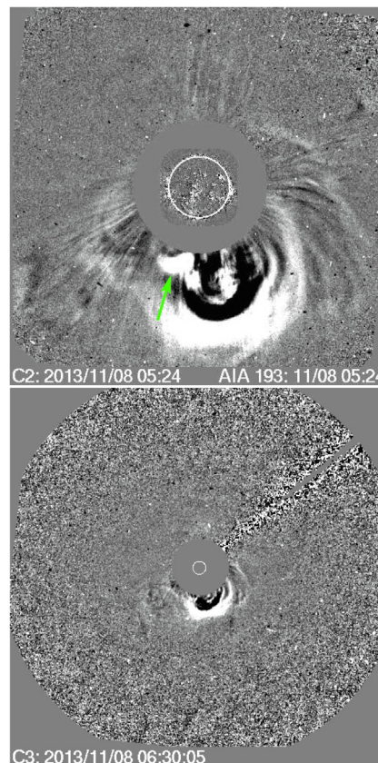
Fig. 6. Solar-MACH plot (prepared with the Solar MAGnetic Connection HAUS tool) shows the field line connecting to the reference longitude of the X1.1 class flare located at S14E15 (indicated with the dashed line, top). SOHO/LASCO C2 observation of the CME at 05:24 UT (middle). A separate plasmoid is visible, indicated with the green arrow. SOHO/LASCO C3 observation of the CME at 06:30 UT (bottom). During 06:00–07:00 UT an IP type II burst was observed by STEREO A and B, but not by Wind.
