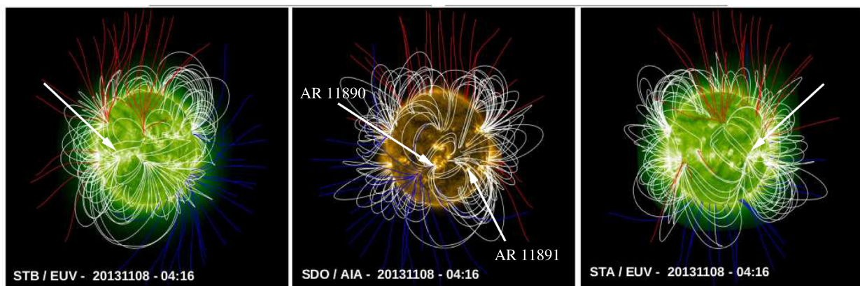
Fig. 5. Magnetic field lines calculated with the potential field source surface (pfss) model, shown in STEREO B, SDO, and STEREO A view. Active regions 11890 and 11891 are marked in the SDO view map, and white arrows mark the erupting region on the far side, near S20W180, in STEREO A and B views. Closed field lines are shown in white and open field lines in red and blue (opposite polarities).
