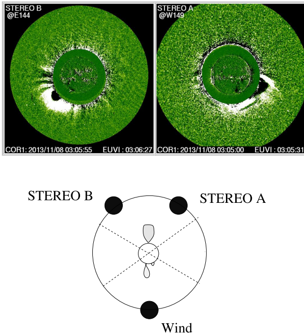
Fig. 4. Dimming regions and the launch of a CME on the far side of the Sun (STEREO A and B observations). The X-class flare on the earthside originated from an active region at E15, the C-class flare was a brightening at W25, and the far side eruption originated from a region near W180. Cartoon shows the locations of these eruptions, together with STEREO A and B positions. SOHO/LASCO and SDO have the same observing direction as Wind. The earthside flaring active regions at low heights were unobservable from STEREO A and B EUV imagers.
