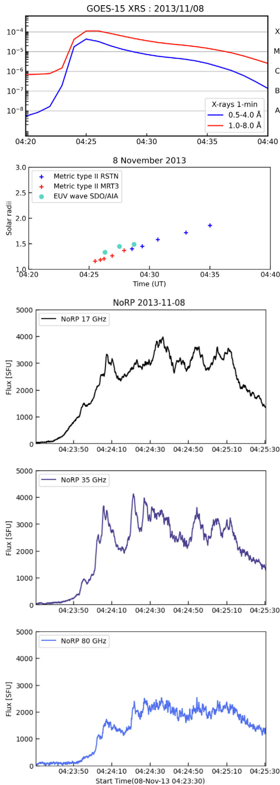
Fig. 2. Top: GOES X-rays from the X1.1 class flare. Middle: Estimated heliocentric distances/heights for the EUV wave (circles), and the metric type II burst (crosses) observed by e-CALLISTO MRT3 at 450–50 MHz and RSTN Learmonth at 180–25 MHz. The calculated radio source heights are listed in Table 2. Bottom three plots: Radio flux densities from the Nobeyama polarimeters at 17, 35, and 80 GHz, in the flare impulsive phase.
