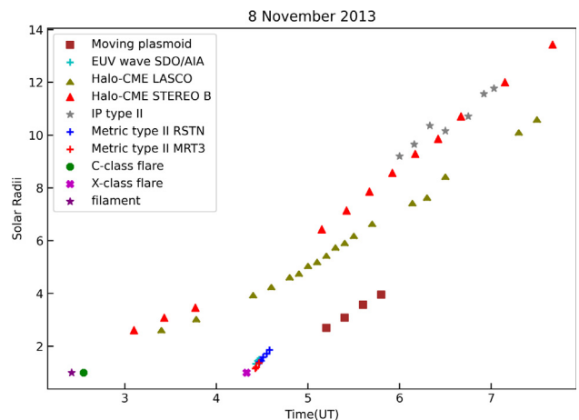
Fig. 9. Measured and calculated heights of all propagating structures. For flares and filament eruption we show their start times.
