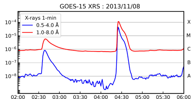
Fig. 1. GOES soft X-ray flux curve shows the C5.7 and X1.1 class flares.
