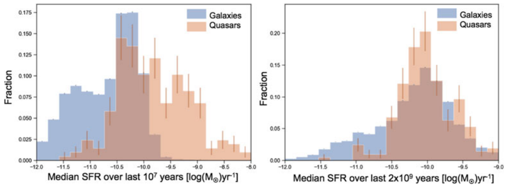
Figure 2. Figure adapted from De Propriis et al. 2020, in prep. Median SFR averaged over 10Myr and 2Gyr for quasar host galaxies ( orange ) and the comparison sample of mass-matched inactive GAMA galaxies ( blue ).
