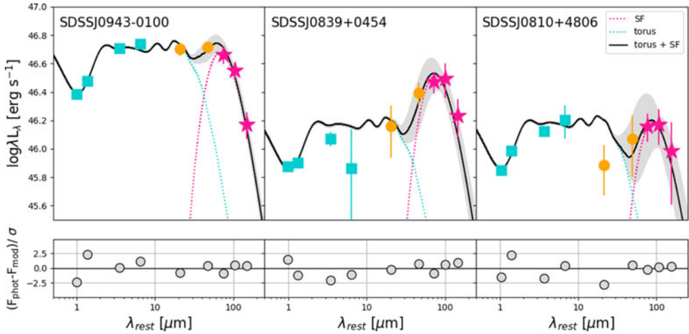
Figure 1. Figure taken from Wethers et al. (2020) . Upper: Best-fit SED template based on the combined WISE (blue squares) + PACS (orange circles) + SPIRE (pink stars) photometry. The total model (black) is comprised of contributions from a hot torus (dotted cyan) and a star forming galaxy (dotted pink). Grey shaded regions denotes the 1\sigma uncertainty in the total model. Lower: Error weighted residuals of the best-fit model.
